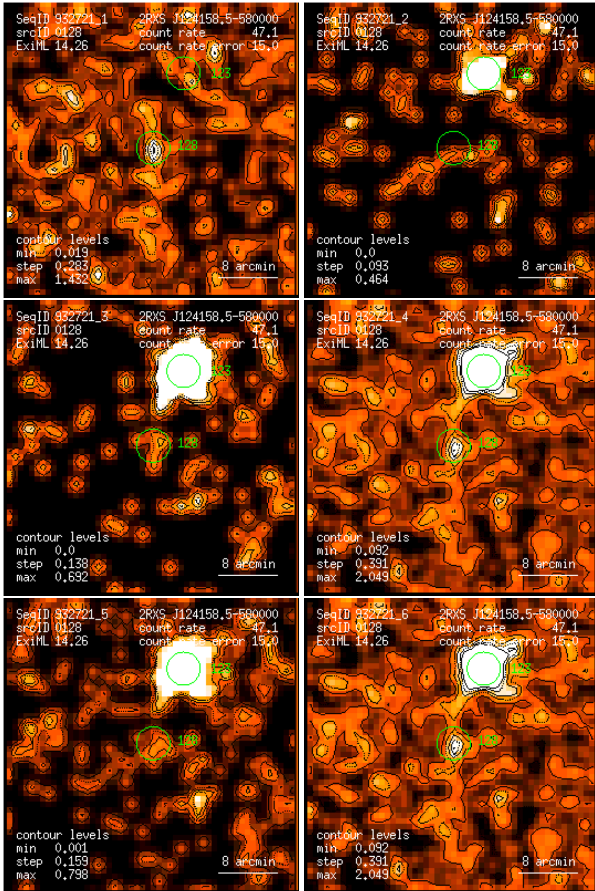
Figure 128: RASS 932721: detection 0128: band rate images, Gaussian filter: (1) PSPC channels 11 – 41, (2) 52 – 90, (3) 91 – 201, (4) 11 – 235, (5) 52 – 201, (6) 11 – 201. Broad band rates in counts/ks. Band rate contour levels in counts/ks/arcmin 2 .
