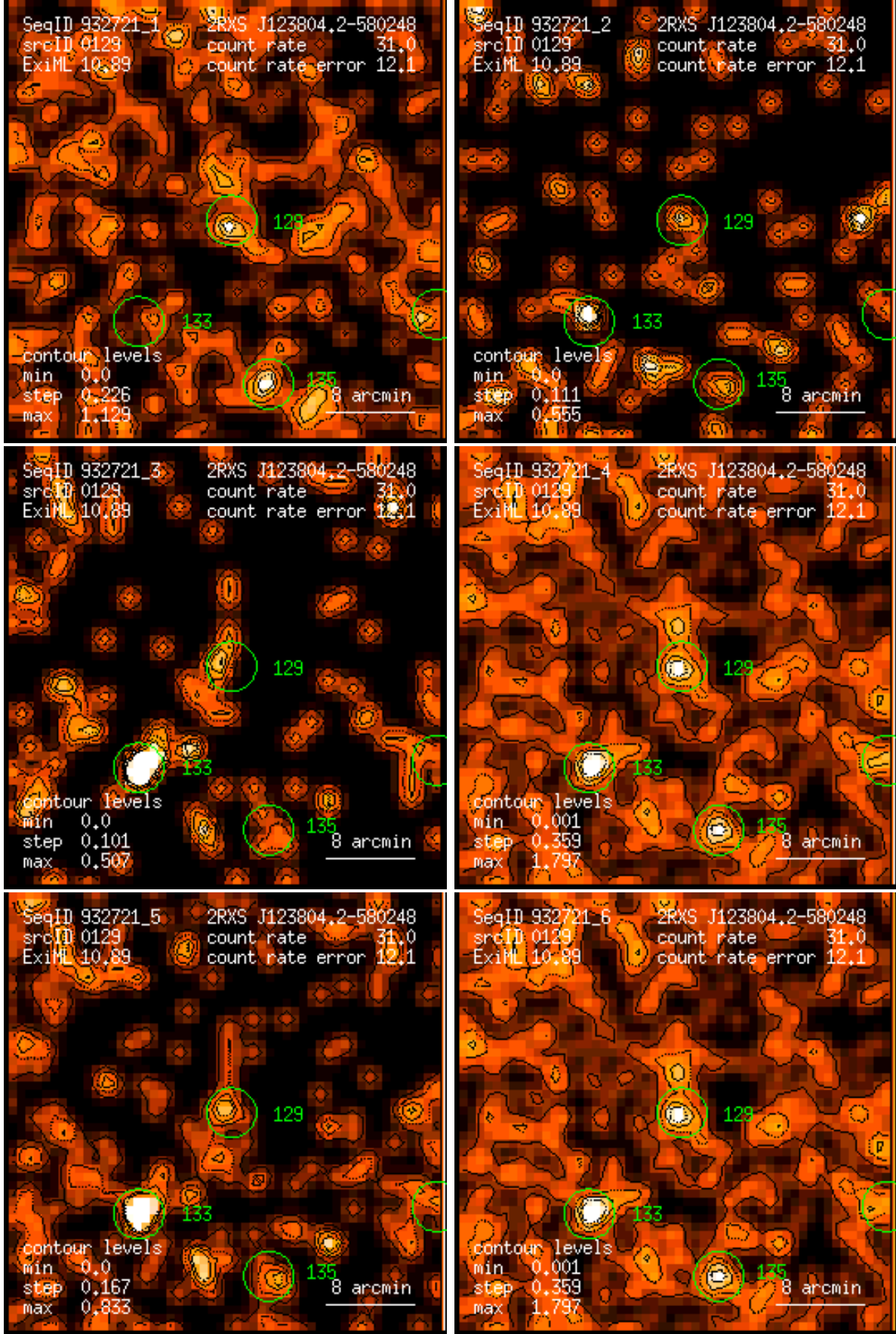
Figure 129: RASS 932721: detection 0129: band rate images, Gaussian filter: (1) PSPC channels 11 – 41, (2) 52 – 90, (3) 91 – 201, (4) 11 – 235, (5) 52 – 201, (6) 11 – 201. Broad band rates in counts/ks. Band rate contour levels in counts/ks/arcmin 2 .
