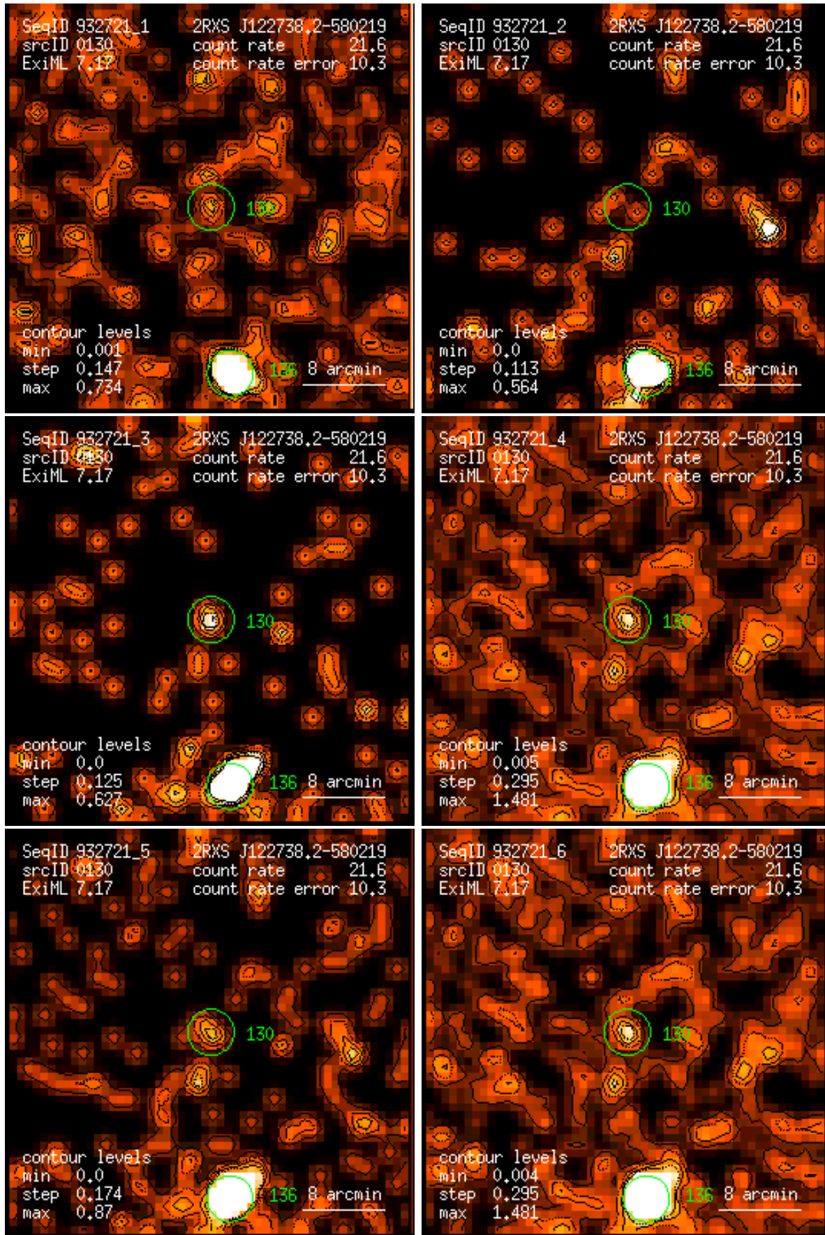
Figure 130: RASS 932721: detection 0130: band rate images, Gaussian filter: (1) PSPC channels 11 – 41, (2) 52 – 90, (3) 91 – 201, (4) 11 – 235, (5) 52 – 201, (6) 11 – 201. Broad band rates in counts/ks. Band rate contour levels in counts/ks/arcmin 2 .
