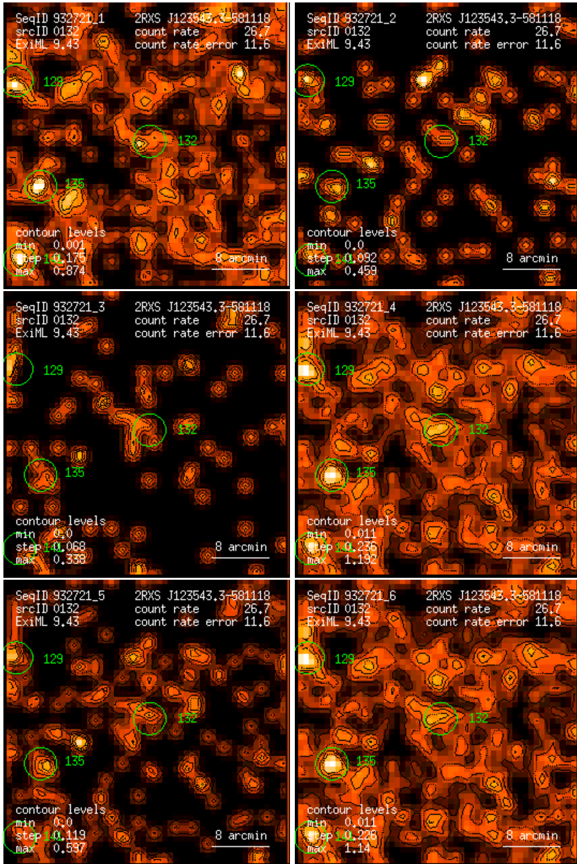
Figure 132: RASS 932721: detection 0132: band rate images, Gaussian filter: (1) PSPC channels 11 – 41, (2) 52 – 90, (3) 91 – 201, (4) 11 – 235, (5) 52 – 201, (6) 11 – 201. Broad band rates in counts/ks. Band rate contour levels in counts/ks/arcmin 2 .
