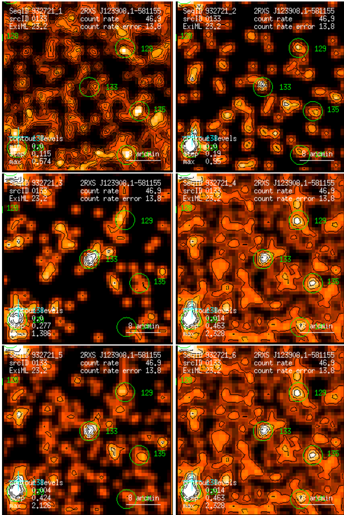
Figure 133: RASS 932721: detection 0133: band rate images, Gaussian filter: (1) PSPC channels 11 – 41, (2) 52 – 90, (3) 91 – 201, (4) 11 – 235, (5) 52 – 201, (6) 11 – 201. Broad band rates in counts/ks. Band rate contour levels in counts/ks/arcmin 2 .
