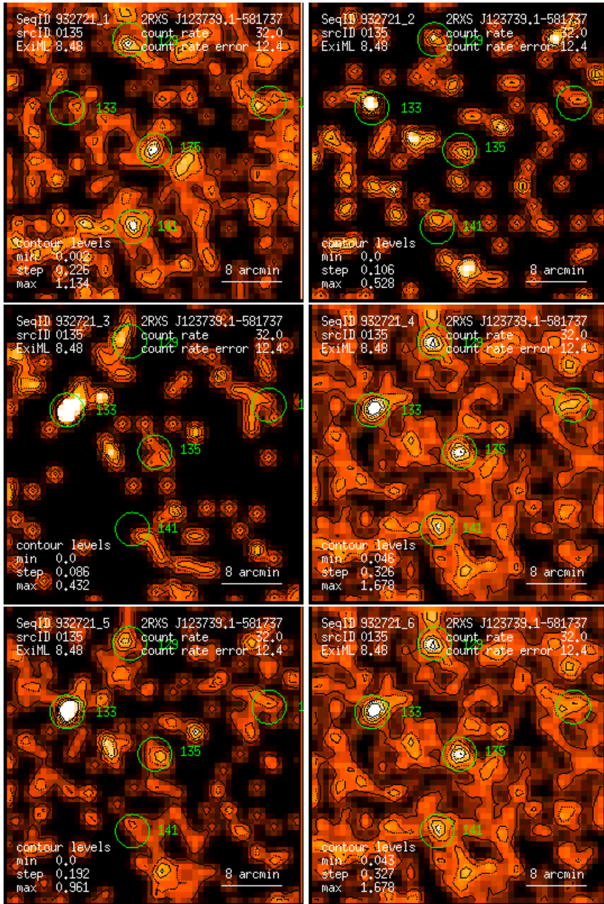
Figure 135: RASS 932721: detection 0135: band rate images, Gaussian filter: (1) PSPC channels 11 – 41, (2) 52 – 90, (3) 91 – 201, (4) 11 – 235, (5) 52 – 201, (6) 11 – 201. Broad band rates in counts/ks. Band rate contour levels in counts/ks/arcmin 2 .
