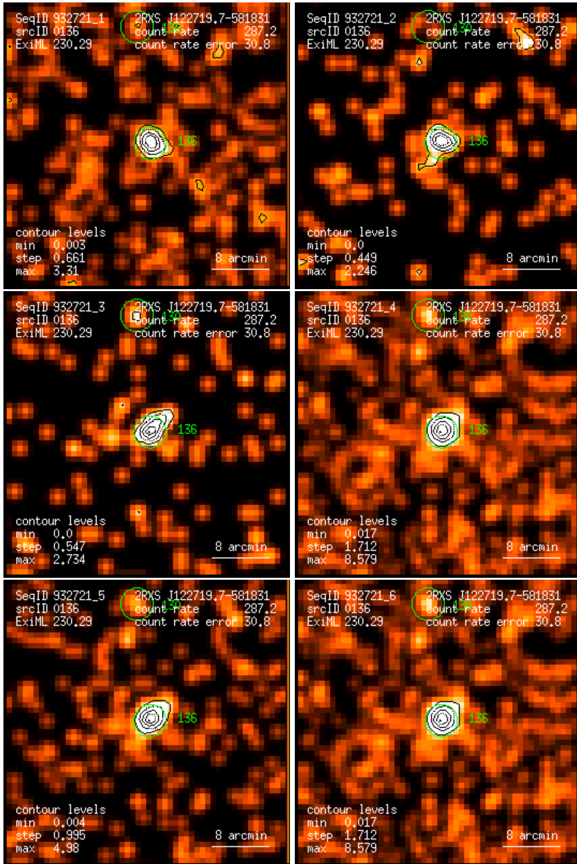
Figure 136: RASS 932721: detection 0136: band rate images, Gaussian filter: (1) PSPC channels 11 – 41, (2) 52 – 90, (3) 91 – 201, (4) 11 – 235, (5) 52 – 201, (6) 11 – 201. Broad band rates in counts/ks. Band rate contour levels in counts/ks/arcmin 2 .
