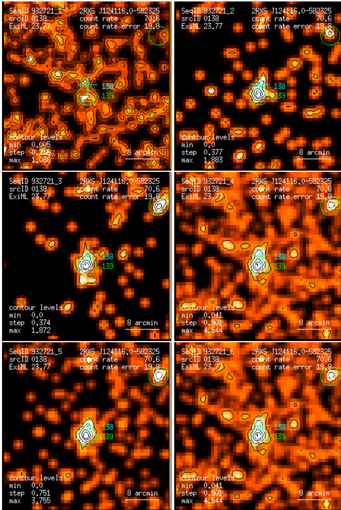
Figure 138: RASS 932721: detection 0138: band rate images, Gaussian filter: (1) PSPC channels 11 – 41, (2) 52 – 90, (3) 91 – 201, (4) 11 – 235, (5) 52 – 201, (6) 11 – 201. Broad band rates in counts/ks. Band rate contour levels in counts/ks/arcmin 2 .
