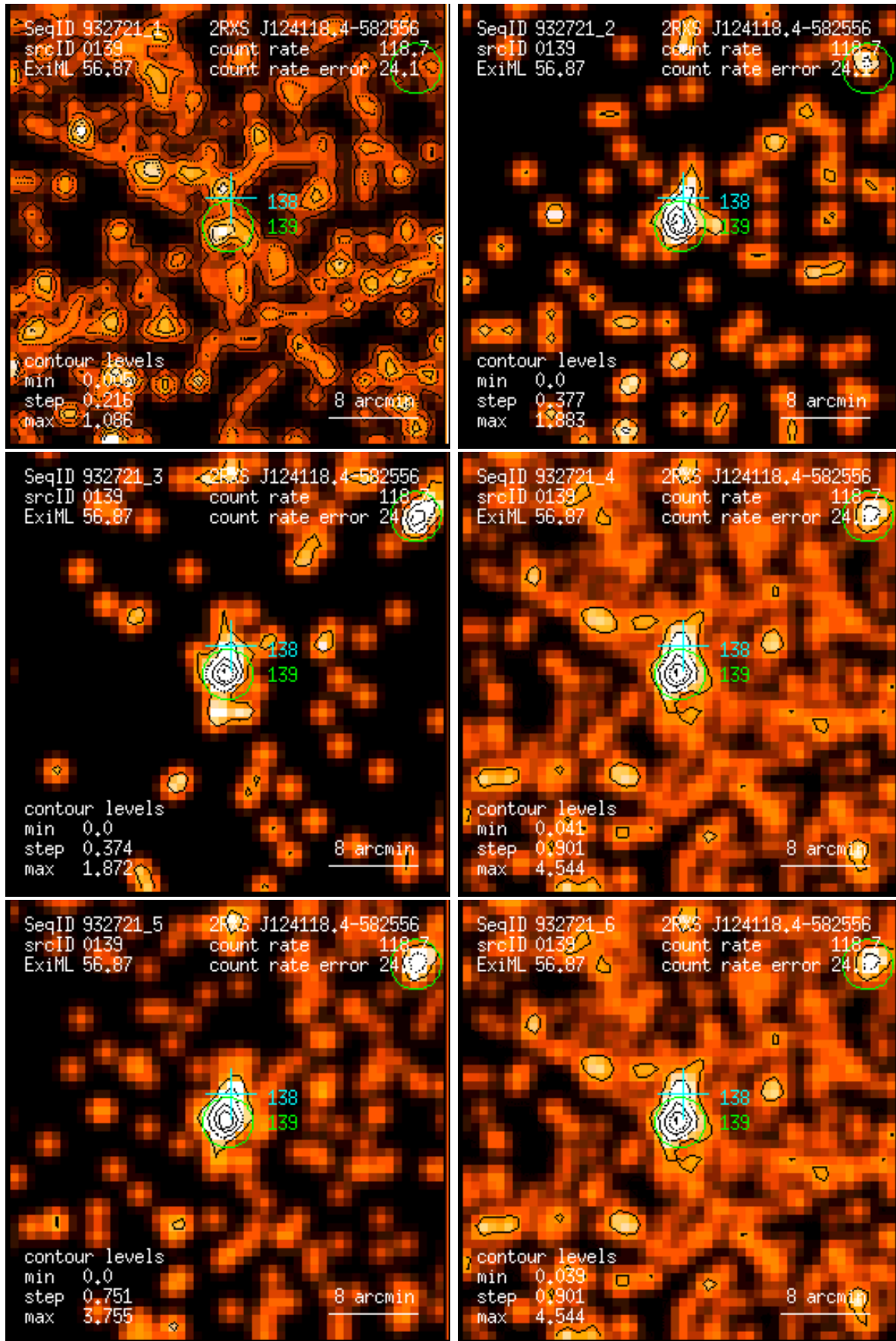
Figure 139: RASS 932721: detection 0139: band rate images, Gaussian filter: (1) PSPC channels 11 – 41, (2) 52 – 90, (3) 91 – 201, (4) 11 – 235, (5) 52 – 201, (6) 11 – 201. Broad band rates in counts/ks. Band rate contour levels in counts/ks/arcmin 2 .
