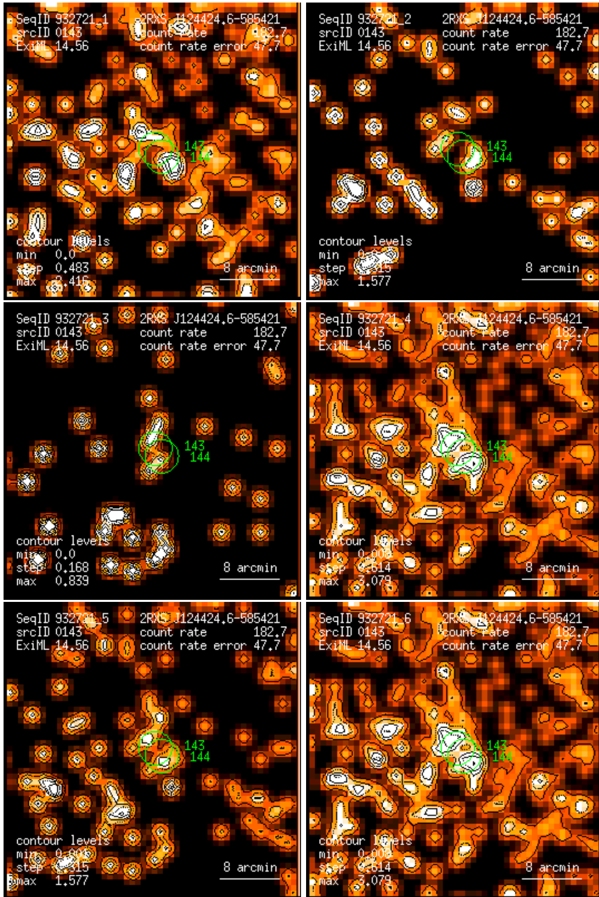
Figure 143: RASS 932721: detection 0143: band rate images, Gaussian filter: (1) PSPC channels 11 – 41, (2) 52 – 90, (3) 91 – 201, (4) 11 – 235, (5) 52 – 201, (6) 11 – 201. Broad band rates in counts/ks. Band rate contour levels in counts/ks/arcmin 2 .
