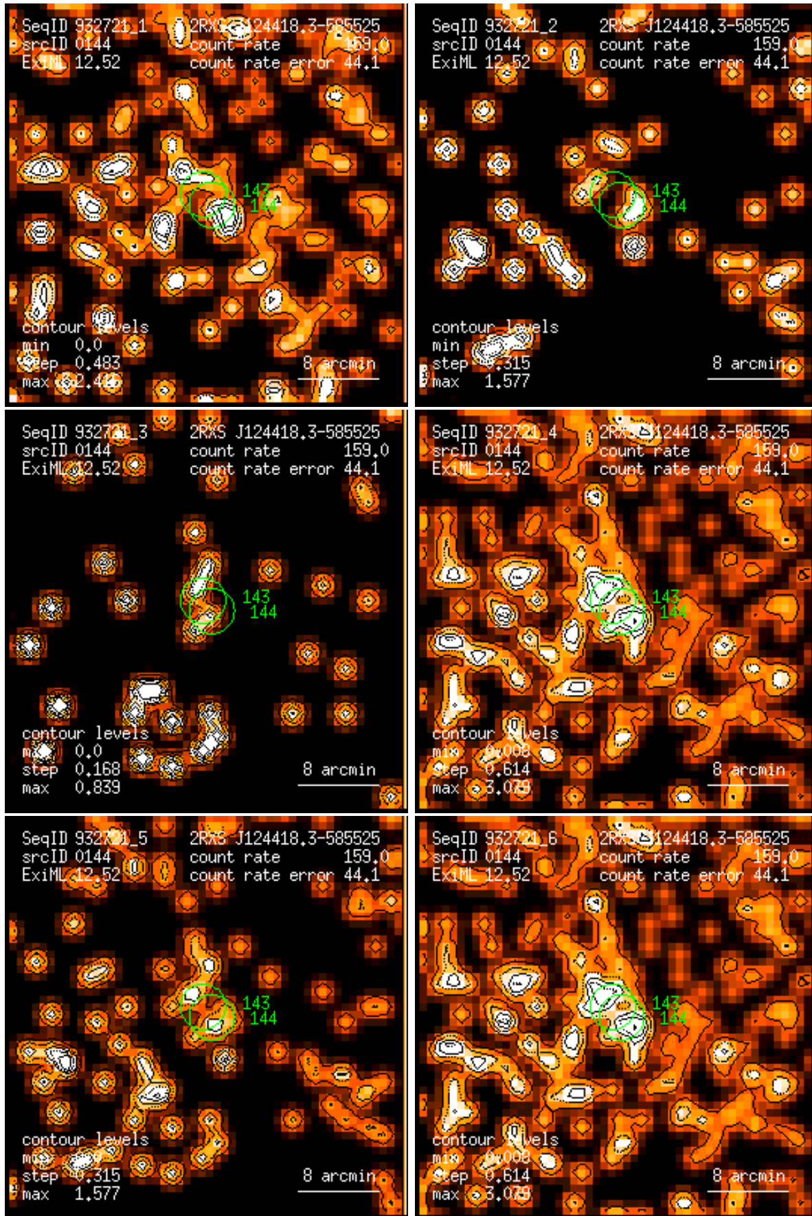
Figure 144: RASS 932721: detection 0144: band rate images, Gaussian filter: (1) PSPC channels 11 – 41, (2) 52 – 90, (3) 91 – 201, (4) 11 – 235, (5) 52 – 201, (6) 11 – 201. Broad band rates in counts/ks. Band rate contour levels in counts/ks/arcmin 2 .
