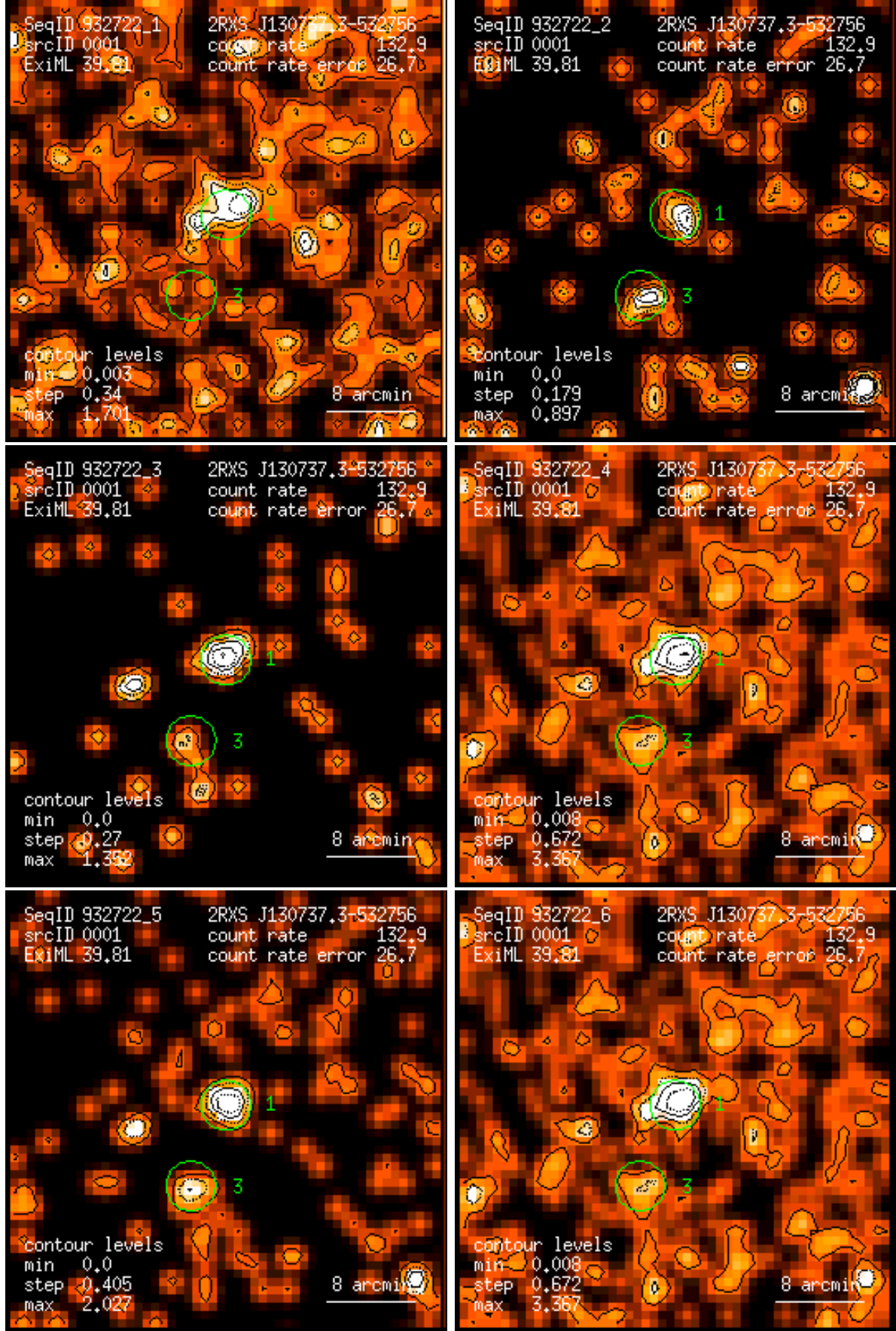
Figure 1: RASS 932722: detection 0001: band rate images, Gaussian filter: (1) PSPC channels 11 – 41, (2) 52 – 90, (3) 91 – 201, (4) 11 – 235, (5) 52 – 201, (6) 11 – 201. Broad band rates in counts/ks. Band rate contour levels in counts/ks/arcmin 2 .
