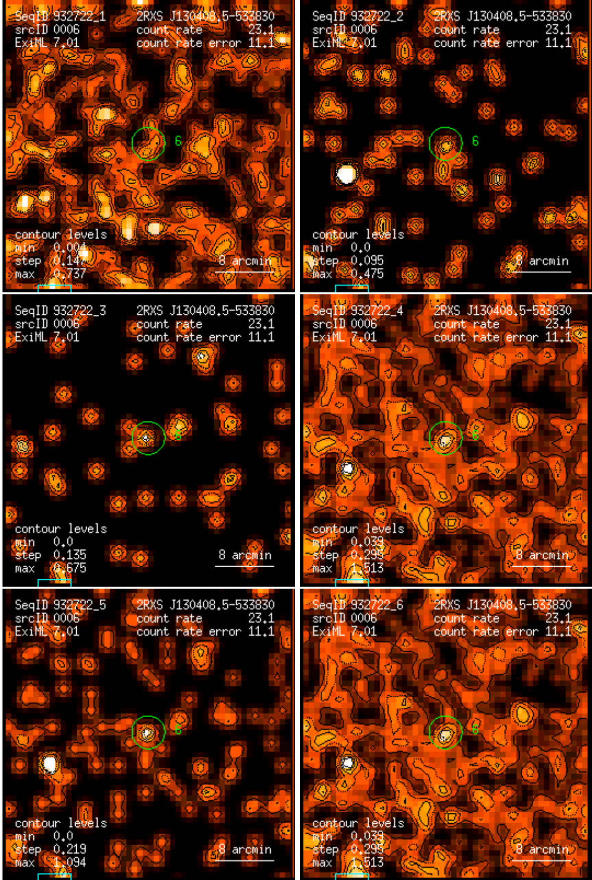
Figure 6: RASS 932722: detection 0006: band rate images, Gaussian filter: (1) PSPC channels 11 – 41, (2) 52 – 90, (3) 91 – 201, (4) 11 – 235, (5) 52 – 201, (6) 11 – 201. Broad band rates in counts/ks. Band rate contour levels in counts/ks/arcmin 2 .
