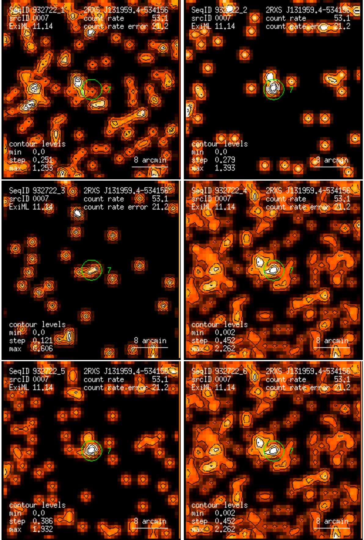
Figure 7: RASS 932722: detection 0007: band rate images, Gaussian filter: (1) PSPC channels 11 – 41, (2) 52 – 90, (3) 91 – 201, (4) 11 – 235, (5) 52 – 201, (6) 11 – 201. Broad band rates in counts/ks. Band rate contour levels in counts/ks/arcmin 2 .
