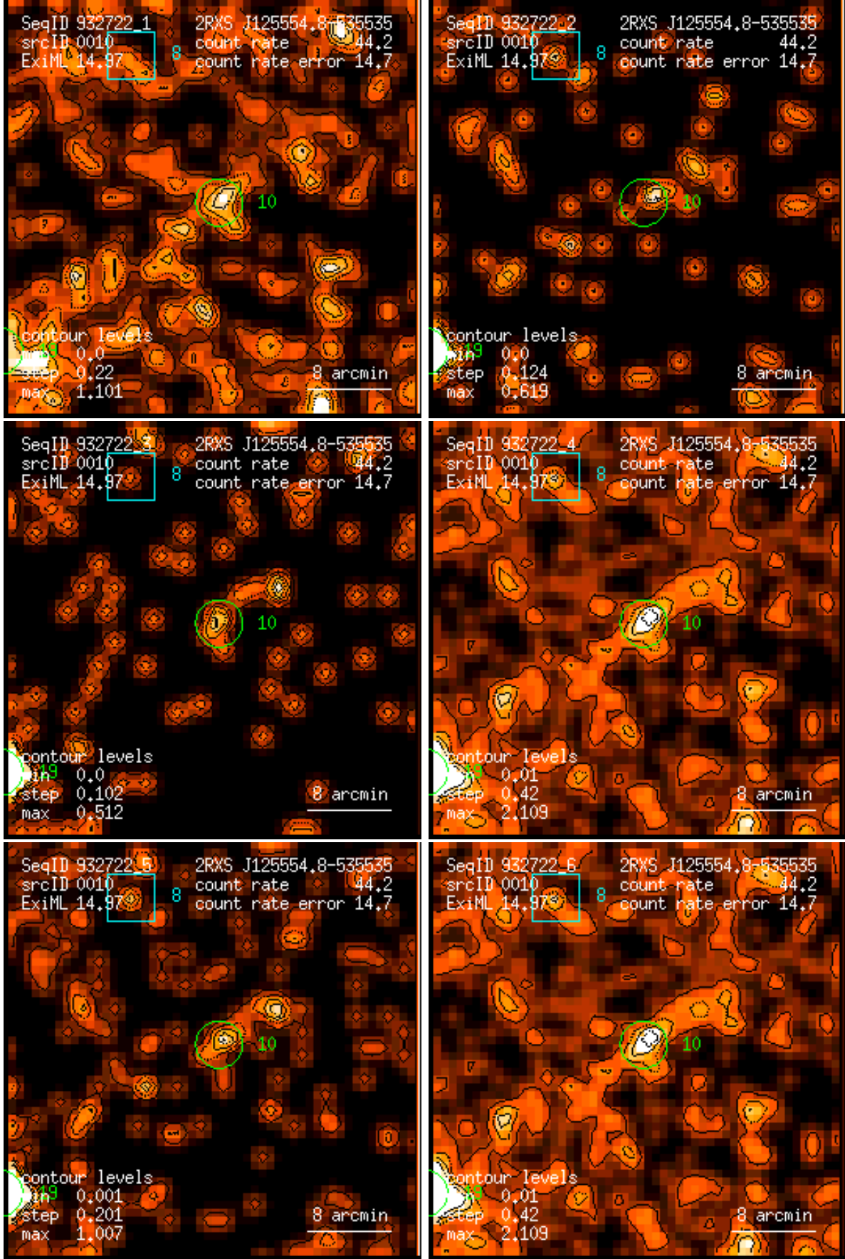
Figure 10: RASS 932722: detection 0010: band rate images, Gaussian filter: (1) PSPC channels 11 – 41, (2) 52 – 90, (3) 91 – 201, (4) 11 – 235, (5) 52 – 201, (6) 11 – 201. Broad band rates in counts/ks. Band rate contour levels in counts/ks/arcmin 2 .
