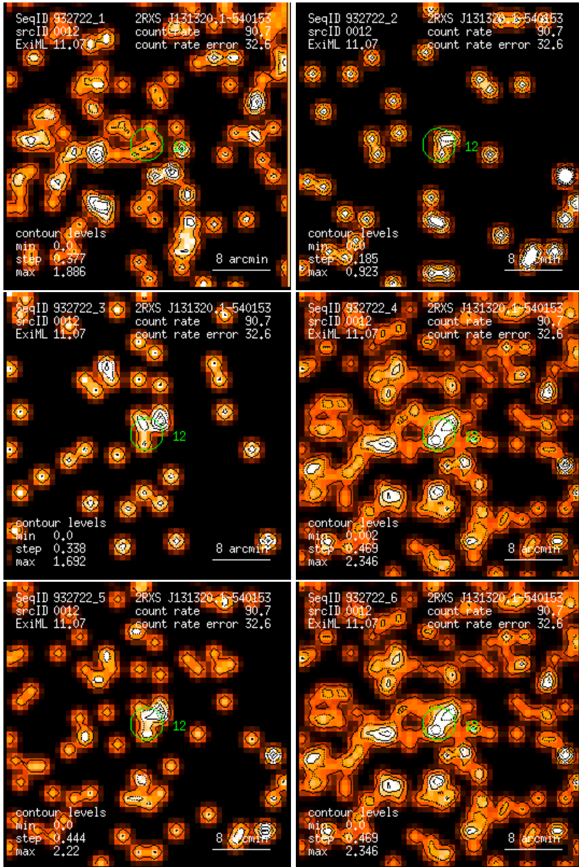
Figure 12: RASS 932722: detection 0012: band rate images, Gaussian filter: (1) PSPC channels 11 – 41, (2) 52 – 90, (3) 91 – 201, (4) 11 – 235, (5) 52 – 201, (6) 11 – 201. Broad band rates in counts/ks. Band rate contour levels in counts/ks/arcmin 2 .
