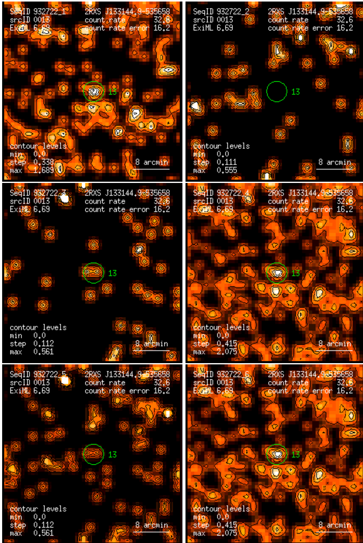
Figure 13: RASS 932722: detection 0013: band rate images, Gaussian filter: (1) PSPC channels 11 – 41, (2) 52 – 90, (3) 91 – 201, (4) 11 – 235, (5) 52 – 201, (6) 11 – 201. Broad band rates in counts/ks. Band rate contour levels in counts/ks/arcmin 2 .
