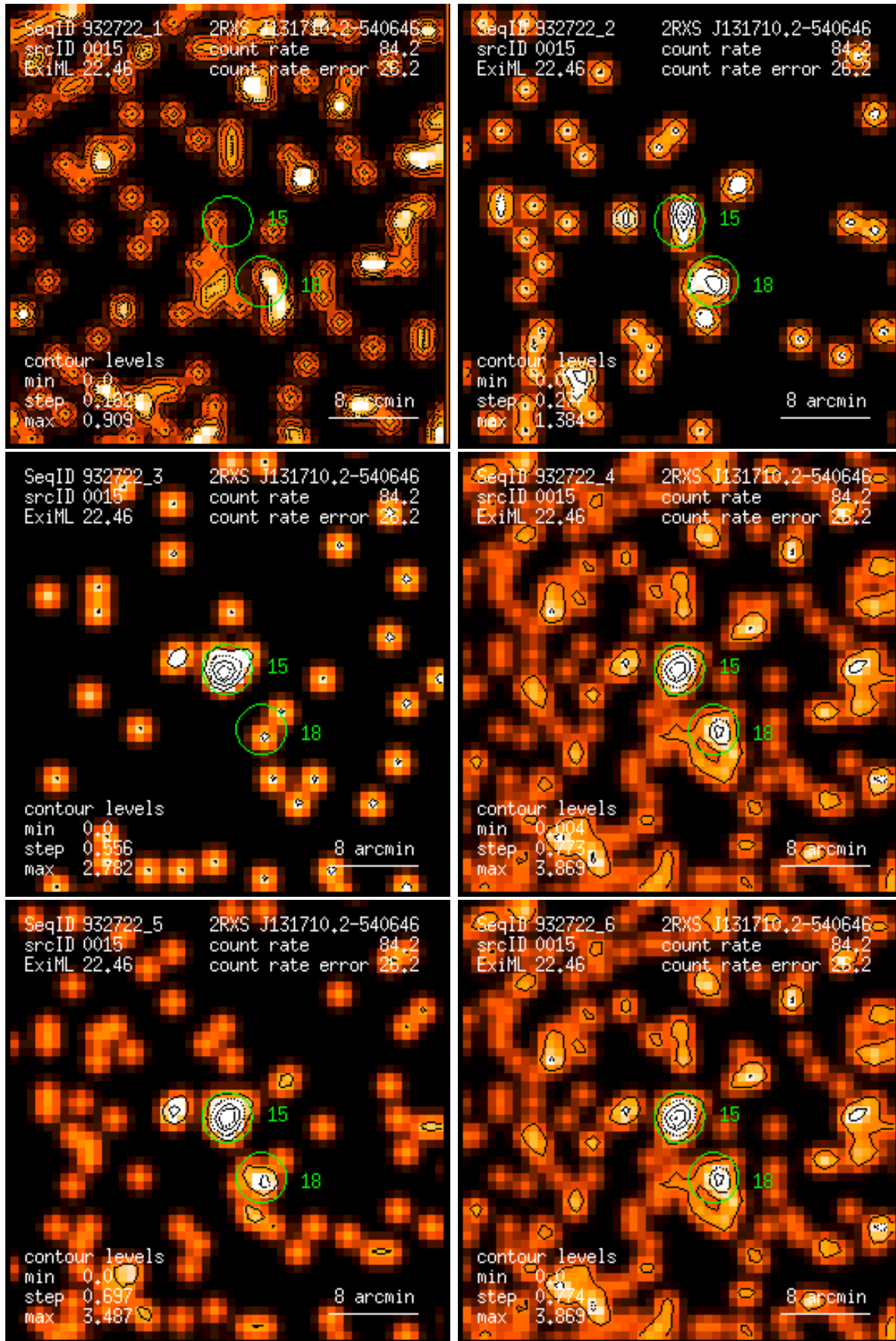
Figure 15: RASS 932722: detection 0015: band rate images, Gaussian filter: (1) PSPC channels 11 – 41, (2) 52 – 90, (3) 91 – 201, (4) 11 – 235, (5) 52 – 201, (6) 11 – 201. Broad band rates in counts/ks. Band rate contour levels in counts/ks/arcmin 2 .
