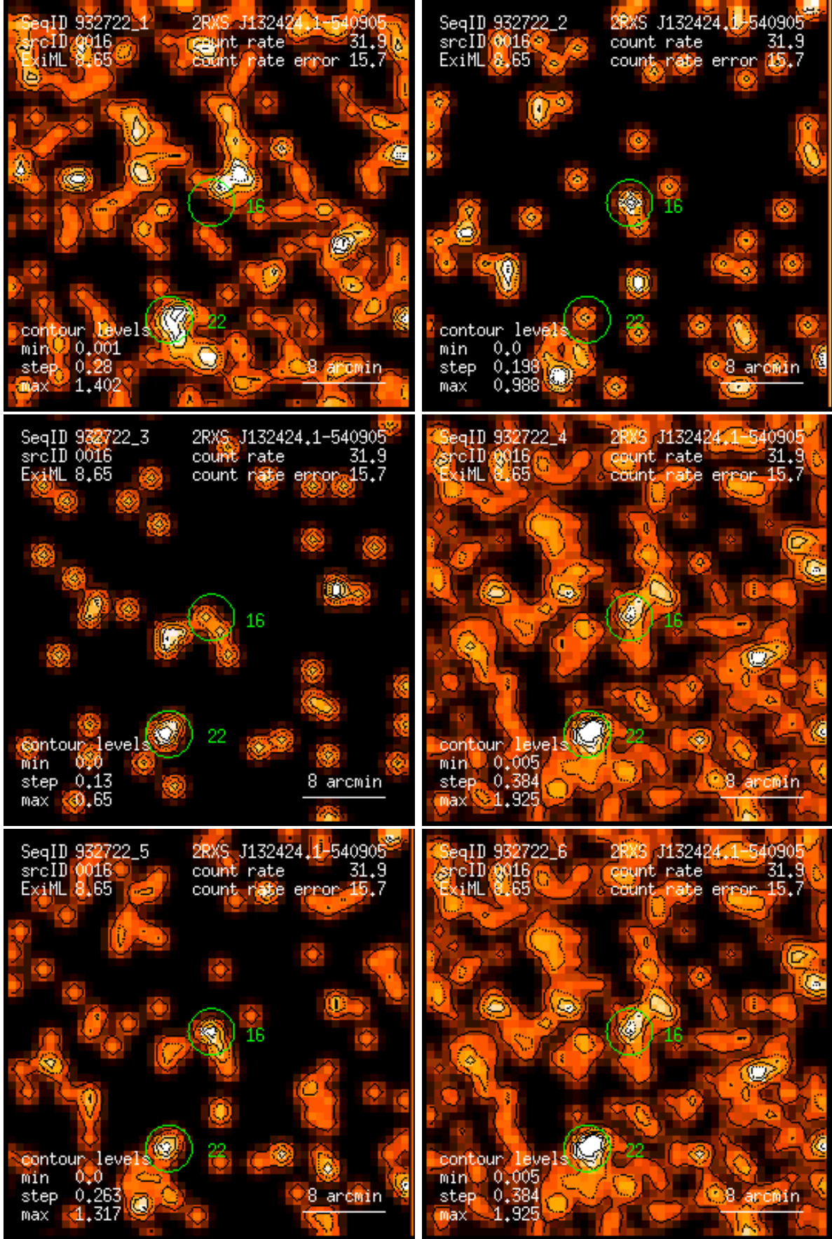
Figure 16: RASS 932722: detection 0016: band rate images, Gaussian filter: (1) PSPC channels 11 – 41, (2) 52 – 90, (3) 91 – 201, (4) 11 – 235, (5) 52 – 201, (6) 11 – 201. Broad band rates in counts/ks. Band rate contour levels in counts/ks/arcmin 2 .
