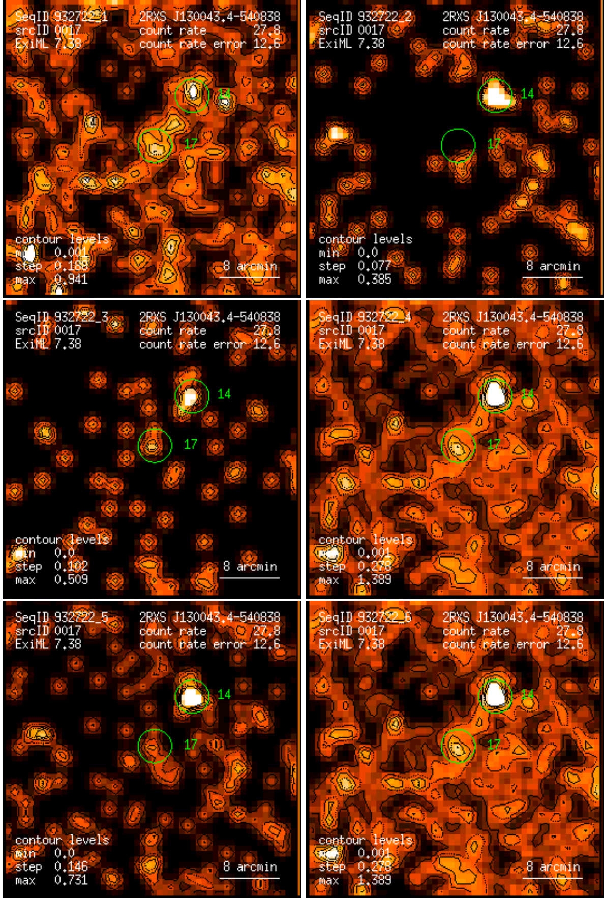
Figure 17: RASS 932722: detection 0017: band rate images, Gaussian filter: (1) PSPC channels 11 – 41, (2) 52 – 90, (3) 91 – 201, (4) 11 – 235, (5) 52 – 201, (6) 11 – 201. Broad band rates in counts/ks. Band rate contour levels in counts/ks/arcmin 2 .
