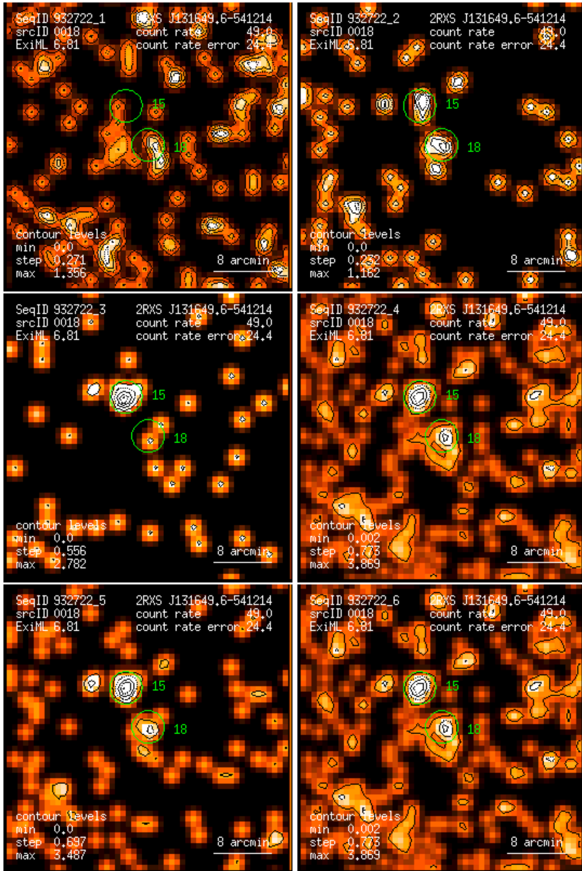
Figure 18: RASS 932722: detection 0018: band rate images, Gaussian filter: (1) PSPC channels 11 – 41, (2) 52 – 90, (3) 91 – 201, (4) 11 – 235, (5) 52 – 201, (6) 11 – 201. Broad band rates in counts/ks. Band rate contour levels in counts/ks/arcmin 2 .
