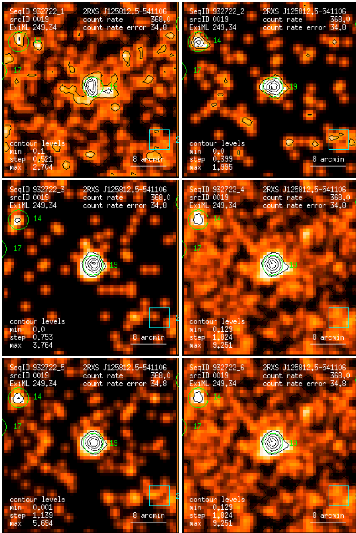
Figure 19: RASS 932722: detection 0019: band rate images, Gaussian filter: (1) PSPC channels 11 – 41, (2) 52 – 90, (3) 91 – 201, (4) 11 – 235, (5) 52 – 201, (6) 11 – 201. Broad band rates in counts/ks. Band rate contour levels in counts/ks/arcmin 2 .
