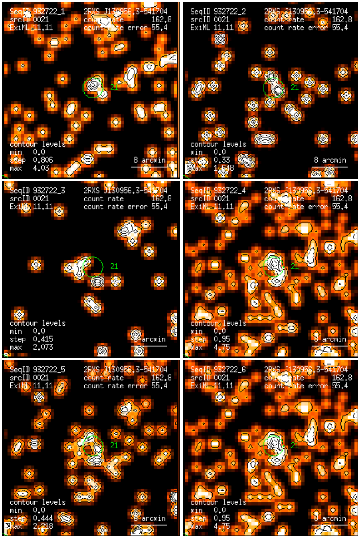
Figure 21: RASS 932722: detection 0021: band rate images, Gaussian filter: (1) PSPC channels 11 – 41, (2) 52 – 90, (3) 91 – 201, (4) 11 – 235, (5) 52 – 201, (6) 11 – 201. Broad band rates in counts/ks. Band rate contour levels in counts/ks/arcmin 2 .
