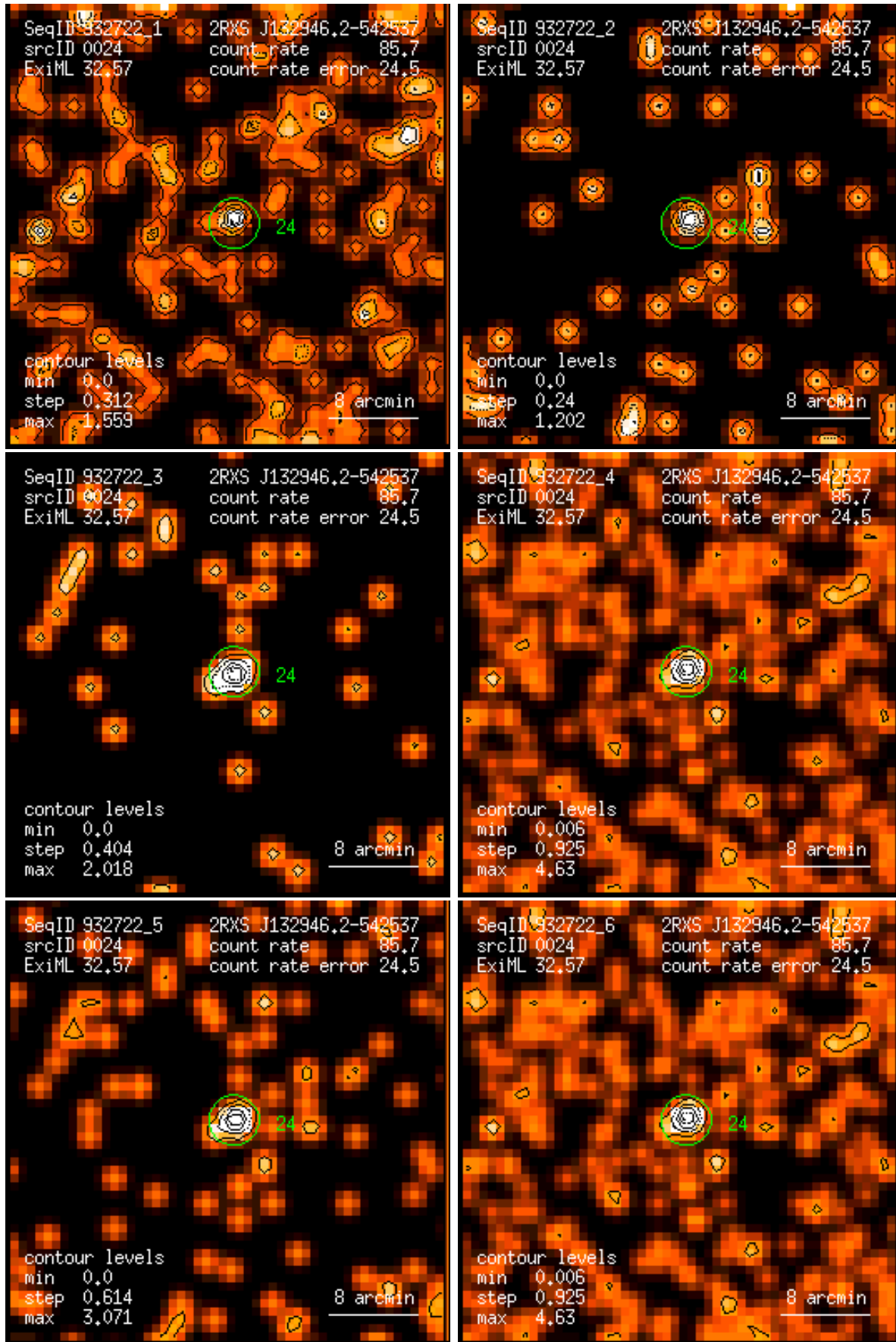
Figure 24: RASS 932722: detection 0024: band rate images, Gaussian filter: (1) PSPC channels 11 – 41, (2) 52 – 90, (3) 91 – 201, (4) 11 – 235, (5) 52 – 201, (6) 11 – 201. Broad band rates in counts/ks. Band rate contour levels in counts/ks/arcmin 2 .
