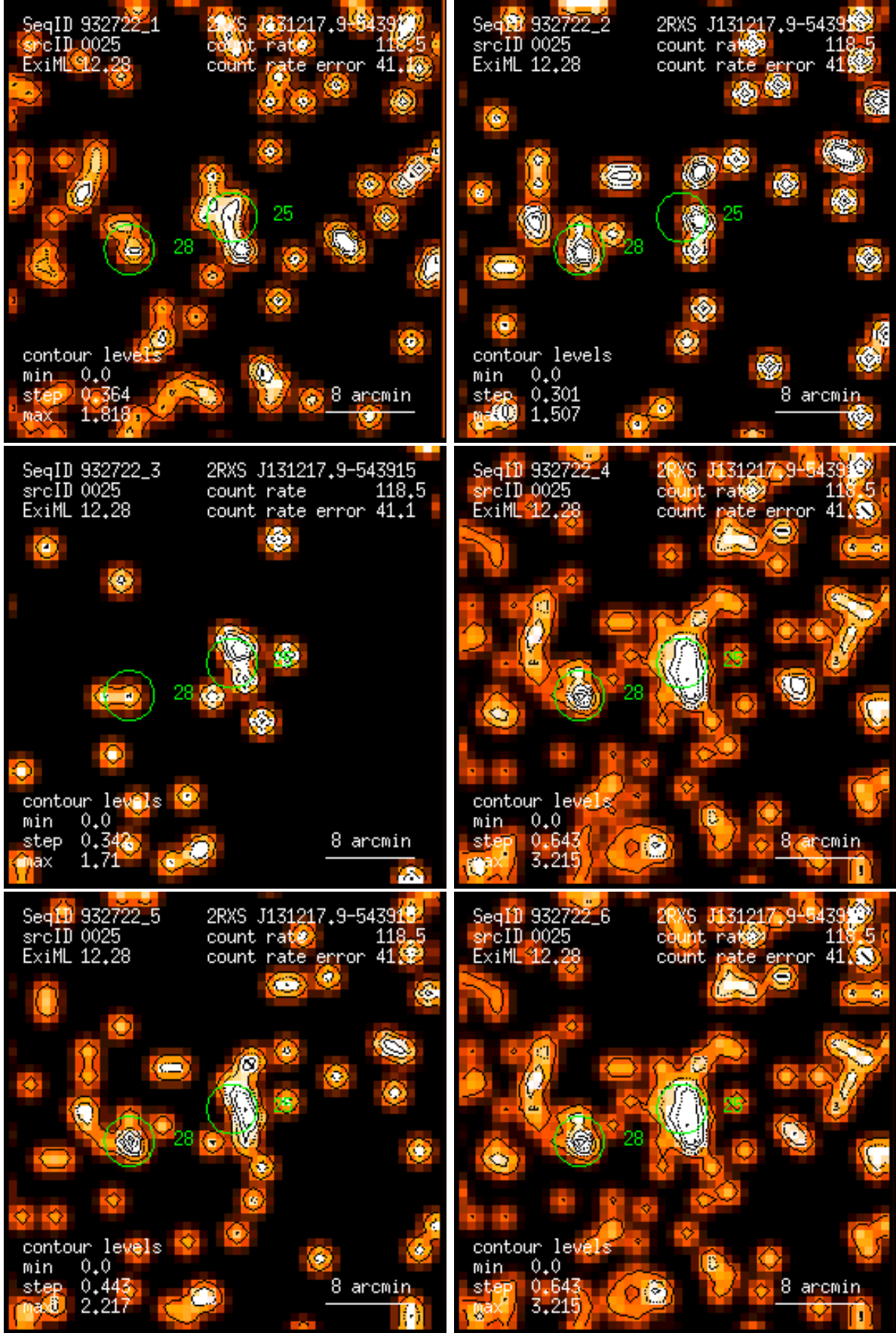
Figure 25: RASS 932722: detection 0025: band rate images, Gaussian filter: (1) PSPC channels 11 – 41, (2) 52 – 90, (3) 91 – 201, (4) 11 – 235, (5) 52 – 201, (6) 11 – 201. Broad band rates in counts/ks. Band rate contour levels in counts/ks/arcmin 2 .
