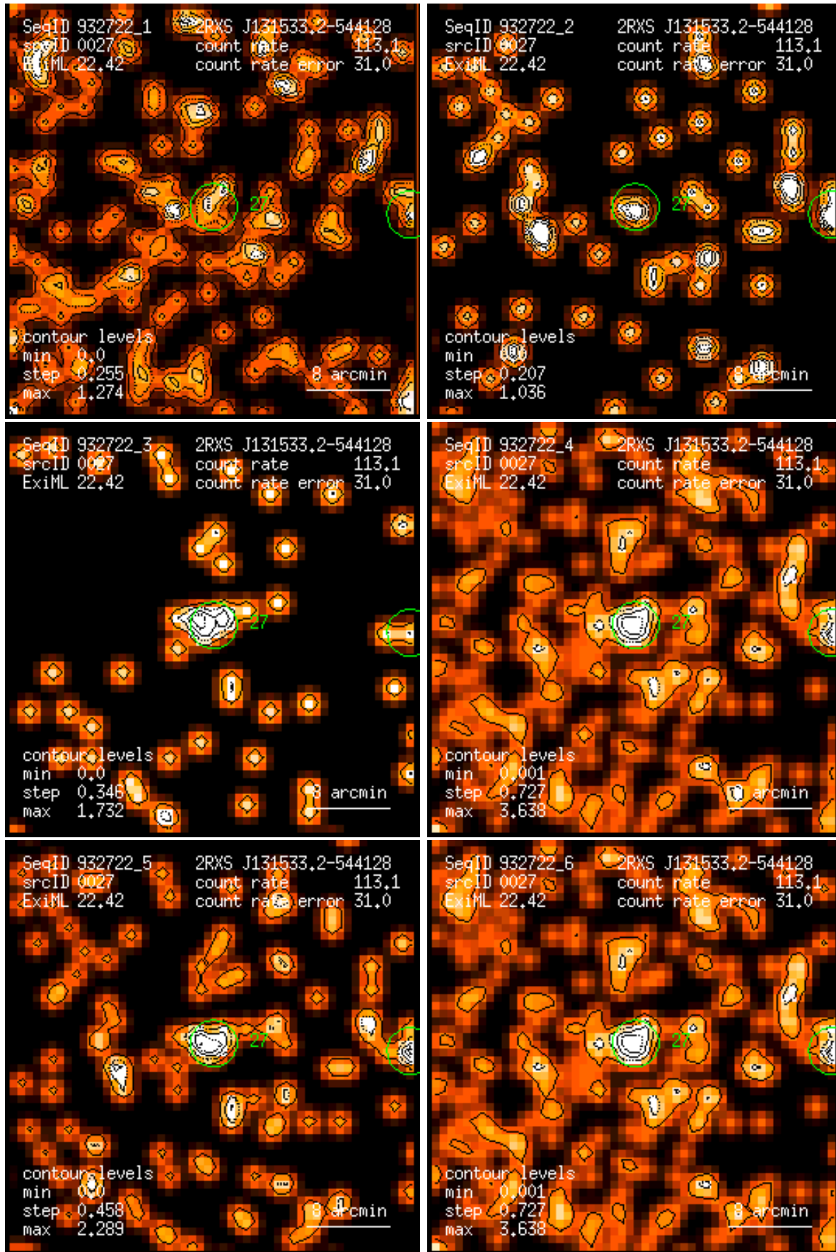
Figure 27: RASS 932722: detection 0027: band rate images, Gaussian filter: (1) PSPC channels 11 – 41, (2) 52 – 90, (3) 91 – 201, (4) 11 – 235, (5) 52 – 201, (6) 11 – 201. Broad band rates in counts/ks. Band rate contour levels in counts/ks/arcmin 2 .
