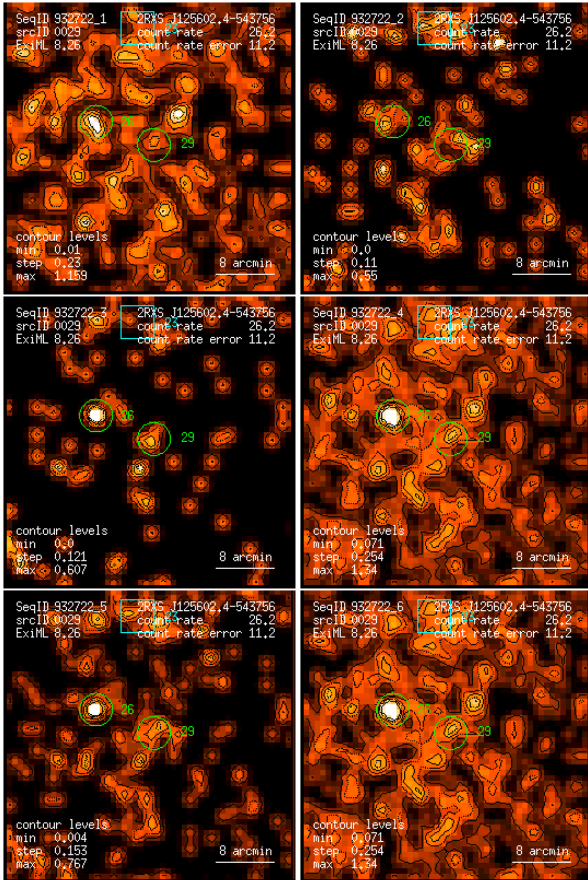
Figure 29: RASS 932722: detection 0029: band rate images, Gaussian filter: (1) PSPC channels 11 – 41, (2) 52 – 90, (3) 91 – 201, (4) 11 – 235, (5) 52 – 201, (6) 11 – 201. Broad band rates in counts/ks. Band rate contour levels in counts/ks/arcmin 2 .
