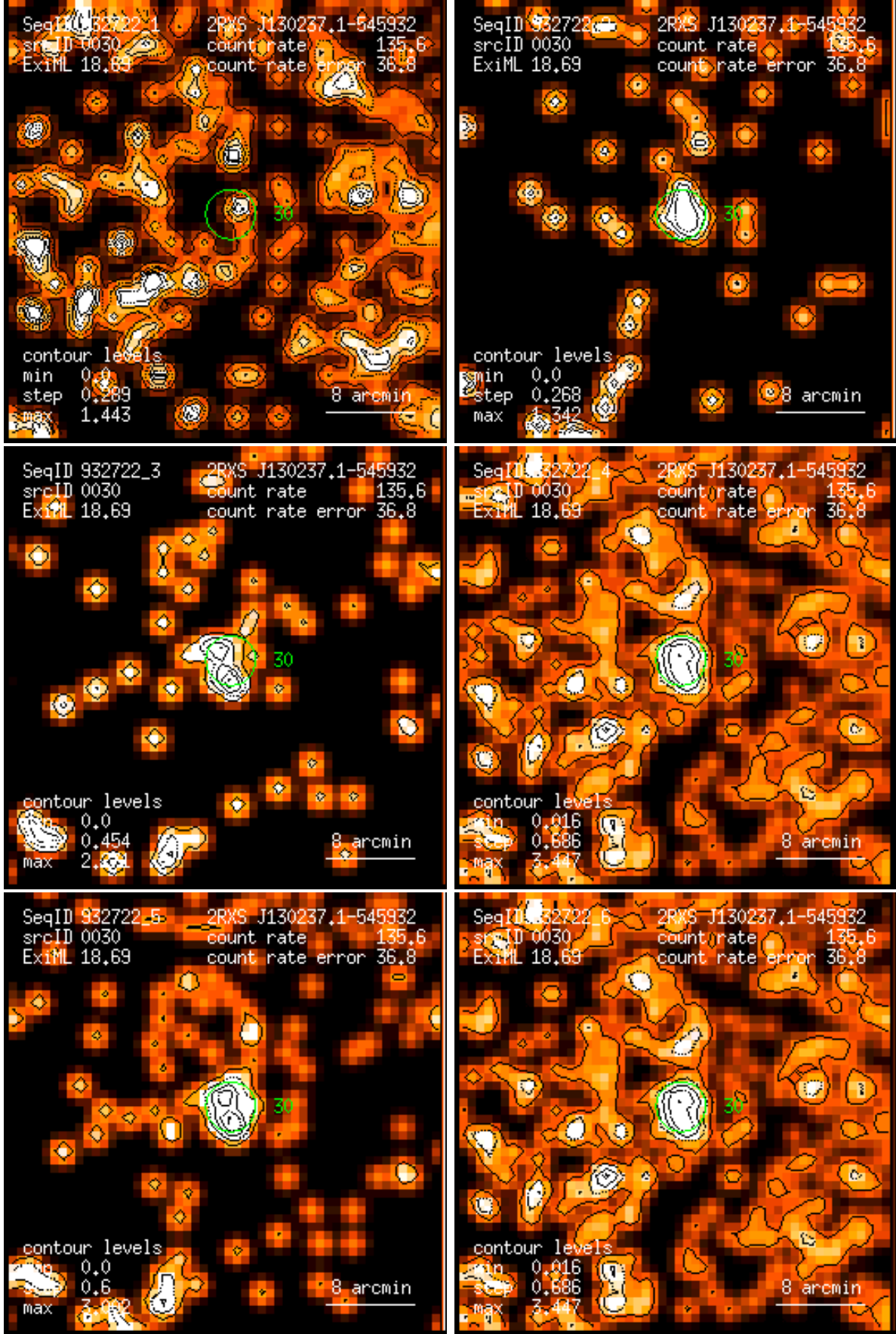
Figure 30: RASS 932722: detection 0030: band rate images, Gaussian filter: (1) PSPC channels 11 – 41, (2) 52 – 90, (3) 91 – 201, (4) 11 – 235, (5) 52 – 201, (6) 11 – 201. Broad band rates in counts/ks. Band rate contour levels in counts/ks/arcmin 2 .
