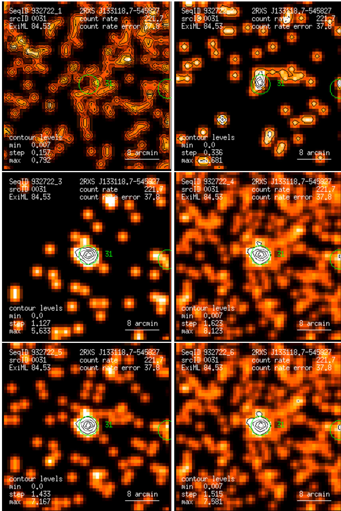
Figure 31: RASS 932722: detection 0031: band rate images, Gaussian filter: (1) PSPC channels 11 – 41, (2) 52 – 90, (3) 91 – 201, (4) 11 – 235, (5) 52 – 201, (6) 11 – 201. Broad band rates in counts/ks. Band rate contour levels in counts/ks/arcmin 2 .
