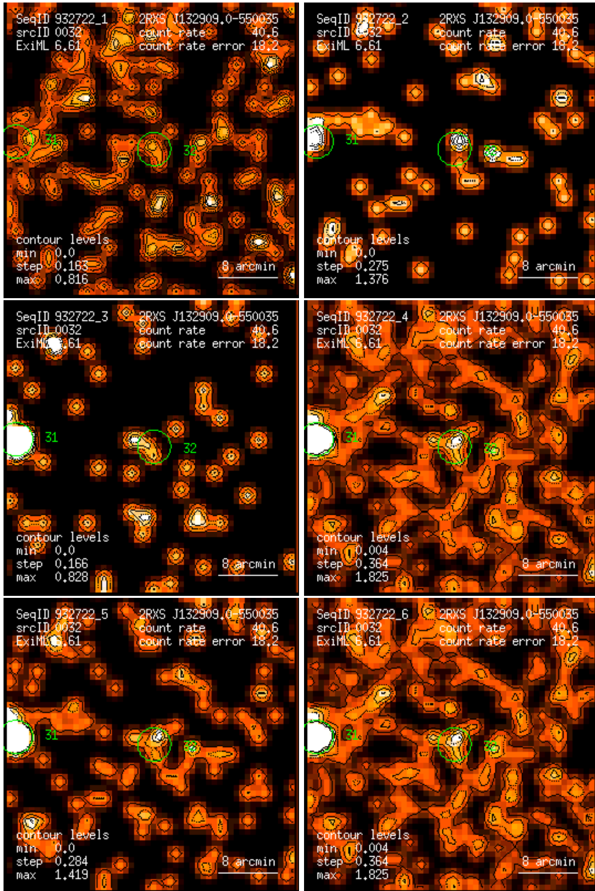
Figure 32: RASS 932722: detection 0032: band rate images, Gaussian filter: (1) PSPC channels 11 – 41, (2) 52 – 90, (3) 91 – 201, (4) 11 – 235, (5) 52 – 201, (6) 11 – 201. Broad band rates in counts/ks. Band rate contour levels in counts/ks/arcmin 2 .
