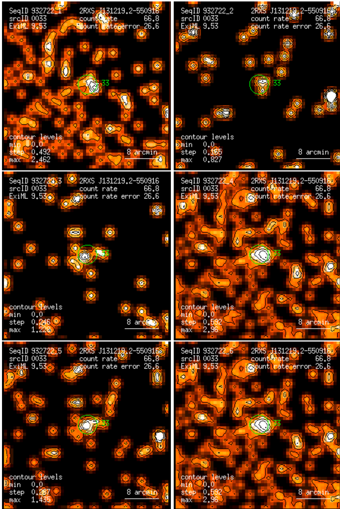
Figure 33: RASS 932722: detection 0033: band rate images, Gaussian filter: (1) PSPC channels 11 – 41, (2) 52 – 90, (3) 91 – 201, (4) 11 – 235, (5) 52 – 201, (6) 11 – 201. Broad band rates in counts/ks. Band rate contour levels in counts/ks/arcmin 2 .
