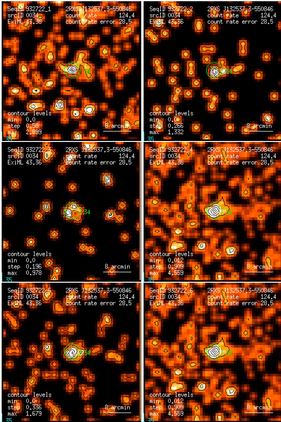
Figure 34: RASS 932722: detection 0034: band rate images, Gaussian filter: (1) PSPC channels 11 – 41, (2) 52 – 90, (3) 91 – 201, (4) 11 – 235, (5) 52 – 201, (6) 11 – 201. Broad band rates in counts/ks. Band rate contour levels in counts/ks/arcmin 2 .
