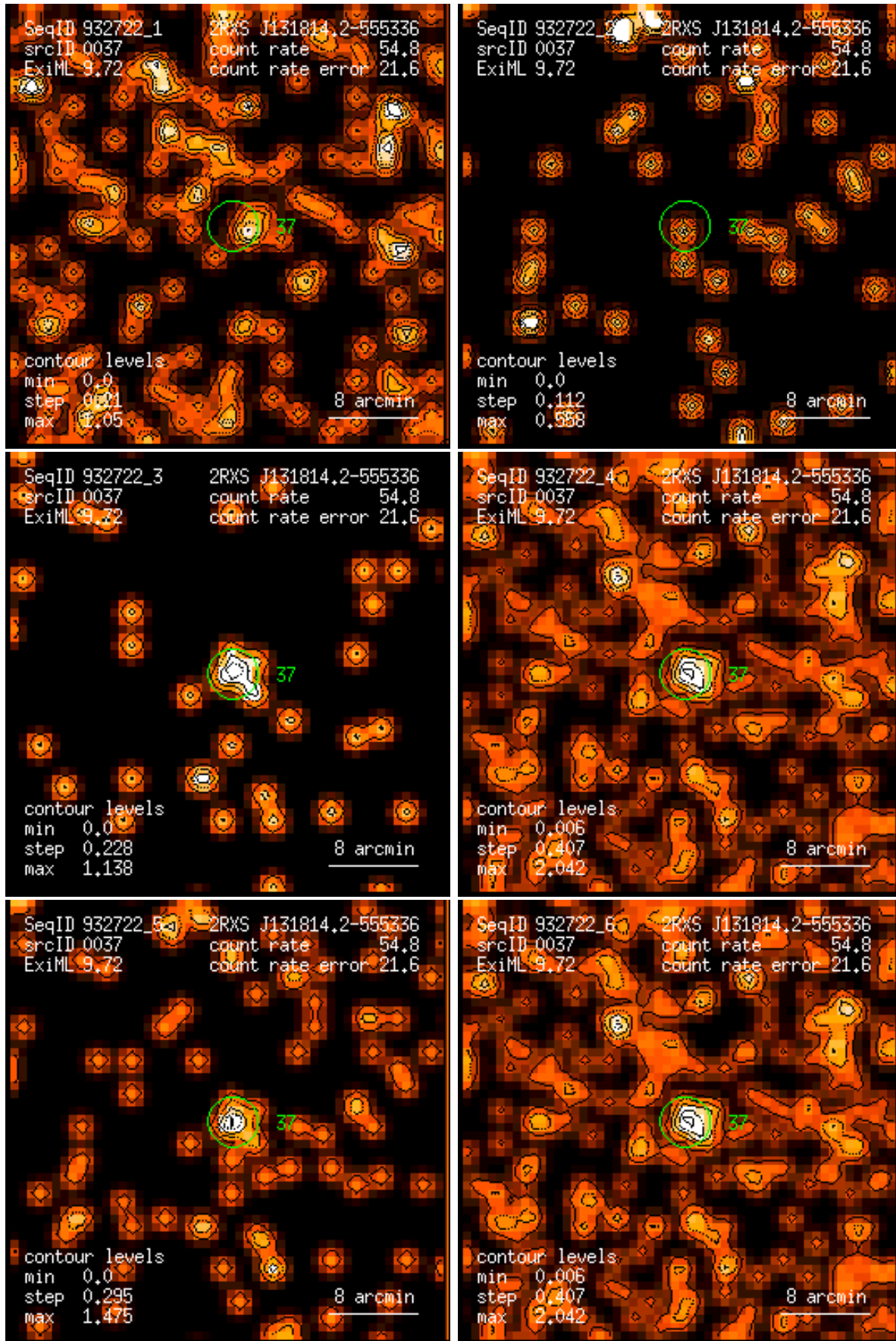
Figure 37: RASS 932722: detection 0037: band rate images, Gaussian filter: (1) PSPC channels 11 – 41, (2) 52 – 90, (3) 91 – 201, (4) 11 – 235, (5) 52 – 201, (6) 11 – 201. Broad band rates in counts/ks. Band rate contour levels in counts/ks/arcmin 2 .
