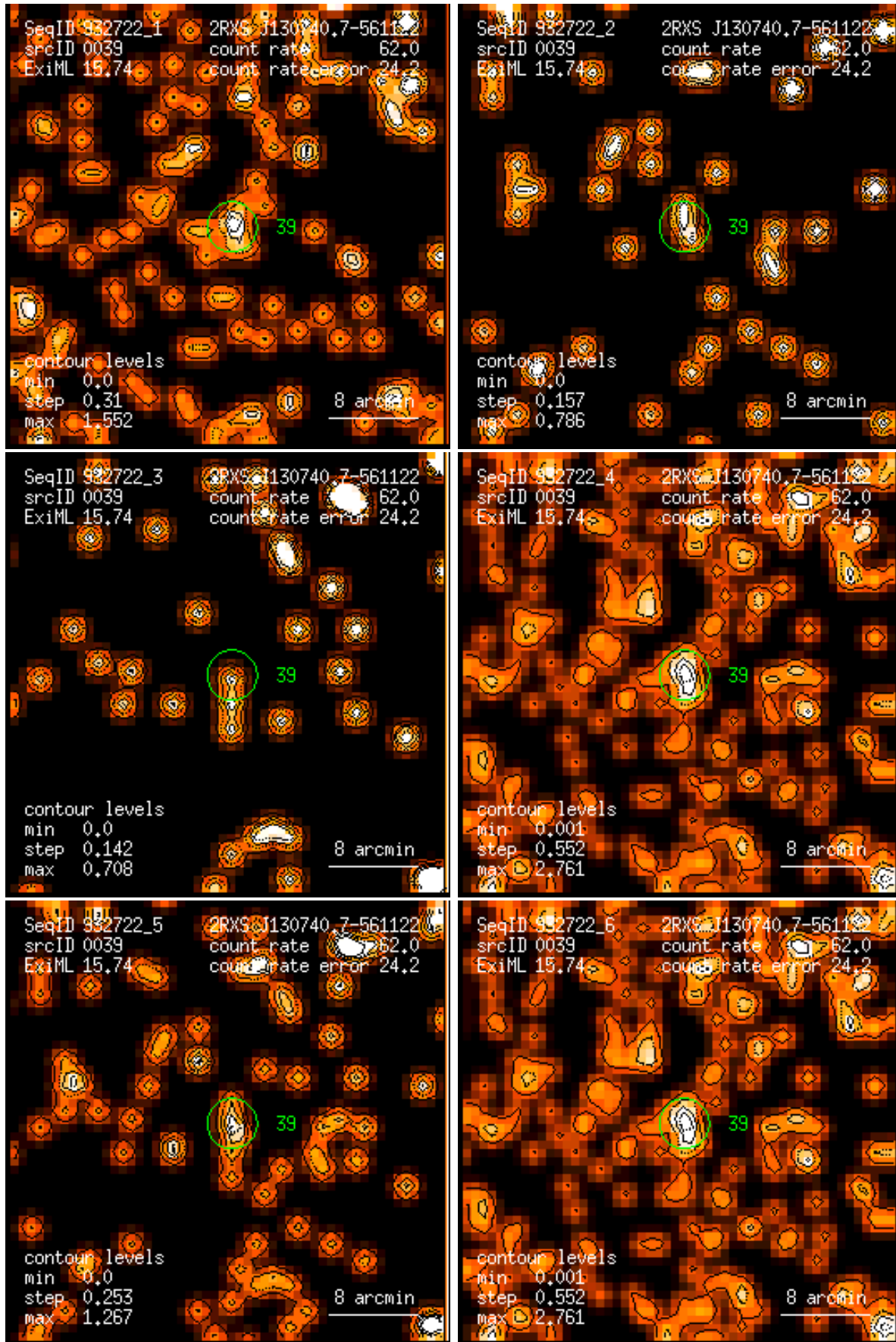
Figure 39: RASS 932722: detection 0039: band rate images, Gaussian filter: (1) PSPC channels 11 – 41, (2) 52 – 90, (3) 91 – 201, (4) 11 – 235, (5) 52 – 201, (6) 11 – 201. Broad band rates in counts/ks. Band rate contour levels in counts/ks/arcmin 2 .
