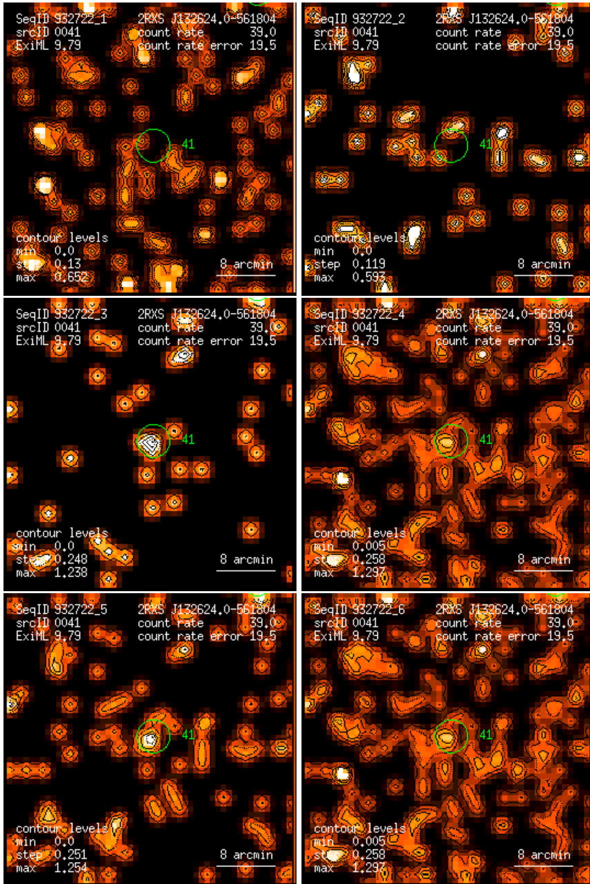
Figure 41: RASS 932722: detection 0041: band rate images, Gaussian filter: (1) PSPC channels 11 – 41, (2) 52 – 90, (3) 91 – 201, (4) 11 – 235, (5) 52 – 201, (6) 11 – 201. Broad band rates in counts/ks. Band rate contour levels in counts/ks/arcmin 2 .
