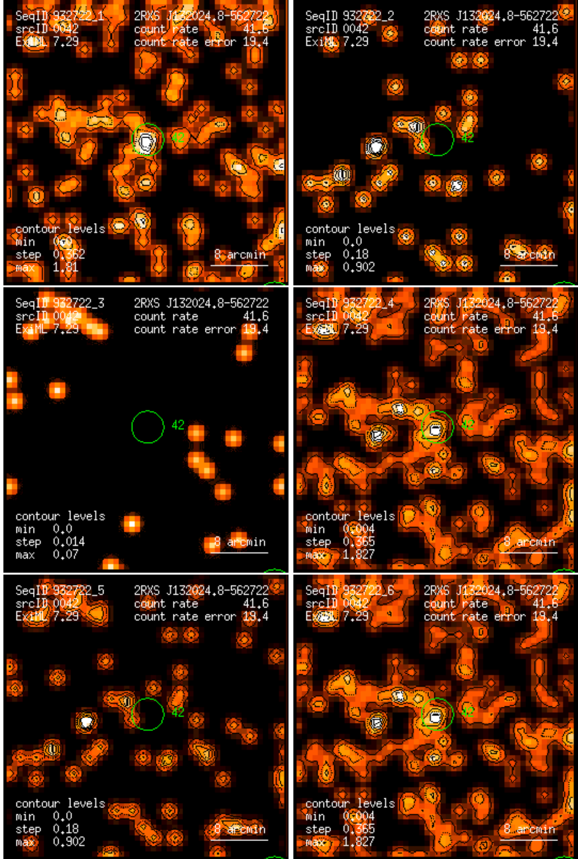
Figure 42: RASS 932722: detection 0042: band rate images, Gaussian filter: (1) PSPC channels 11 – 41, (2) 52 – 90, (3) 91 – 201, (4) 11 – 235, (5) 52 – 201, (6) 11 – 201. Broad band rates in counts/ks. Band rate contour levels in counts/ks/arcmin 2 .
