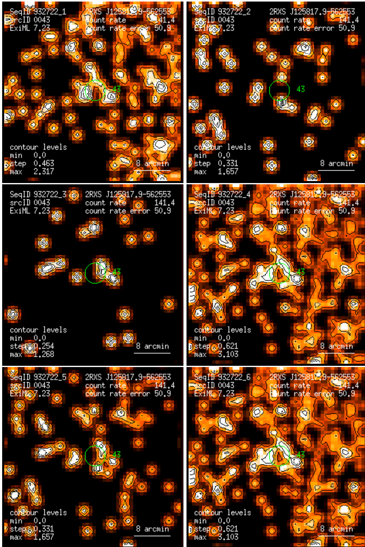
Figure 43: RASS 932722: detection 0043: band rate images, Gaussian filter: (1) PSPC channels 11 – 41, (2) 52 – 90, (3) 91 – 201, (4) 11 – 235, (5) 52 – 201, (6) 11 – 201. Broad band rates in counts/ks. Band rate contour levels in counts/ks/arcmin 2 .
