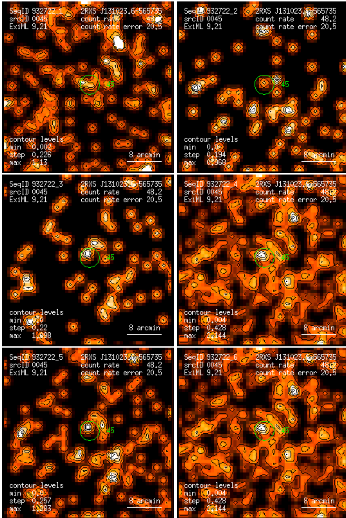
Figure 45: RASS 932722: detection 0045: band rate images, Gaussian filter: (1) PSPC channels 11 – 41, (2) 52 – 90, (3) 91 – 201, (4) 11 – 235, (5) 52 – 201, (6) 11 – 201. Broad band rates in counts/ks. Band rate contour levels in counts/ks/arcmin 2 .
