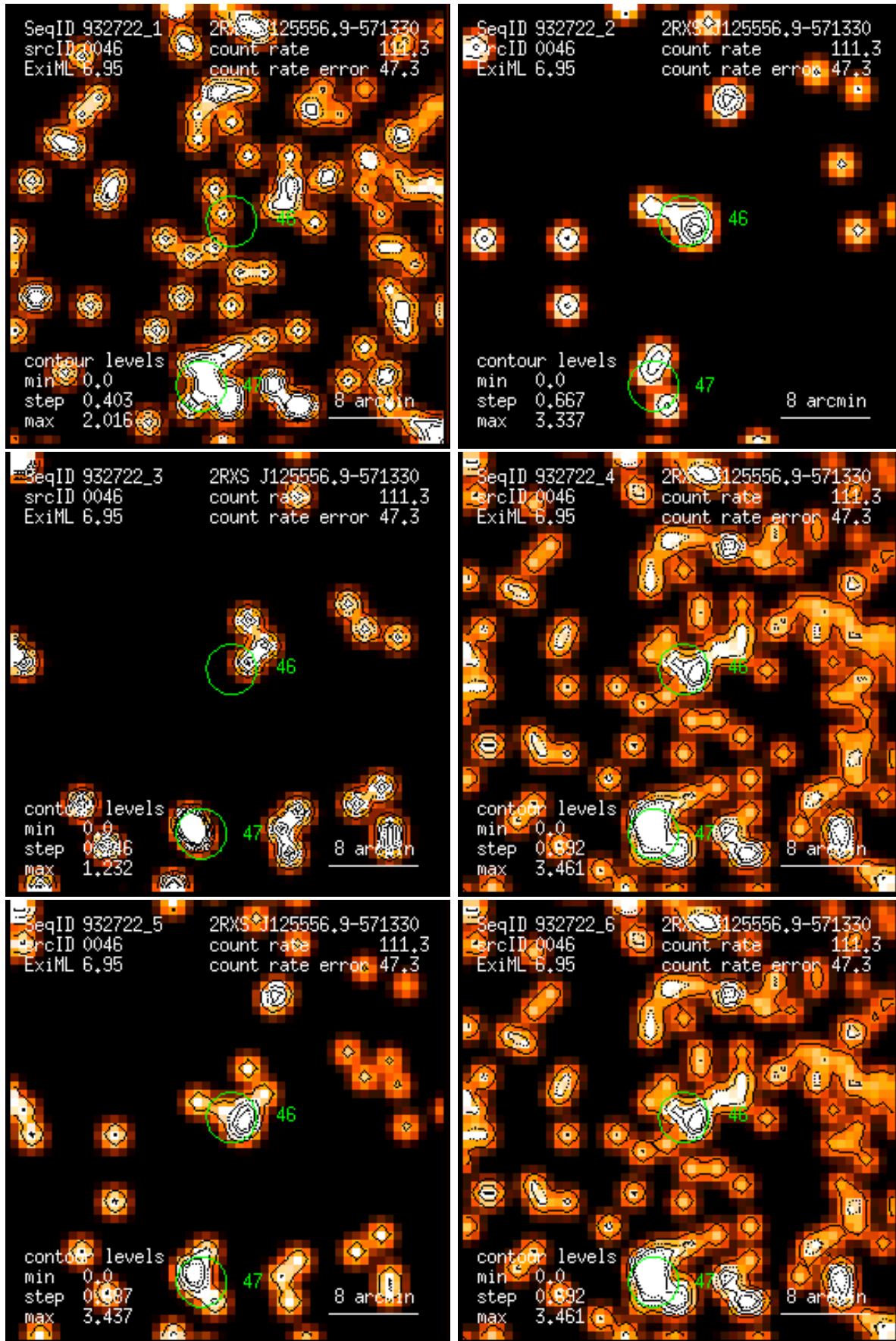
Figure 46: RASS 932722: detection 0046: band rate images, Gaussian filter: (1) PSPC channels 11 – 41, (2) 52 – 90, (3) 91 – 201, (4) 11 – 235, (5) 52 – 201, (6) 11 – 201. Broad band rates in counts/ks. Band rate contour levels in counts/ks/arcmin 2 .
