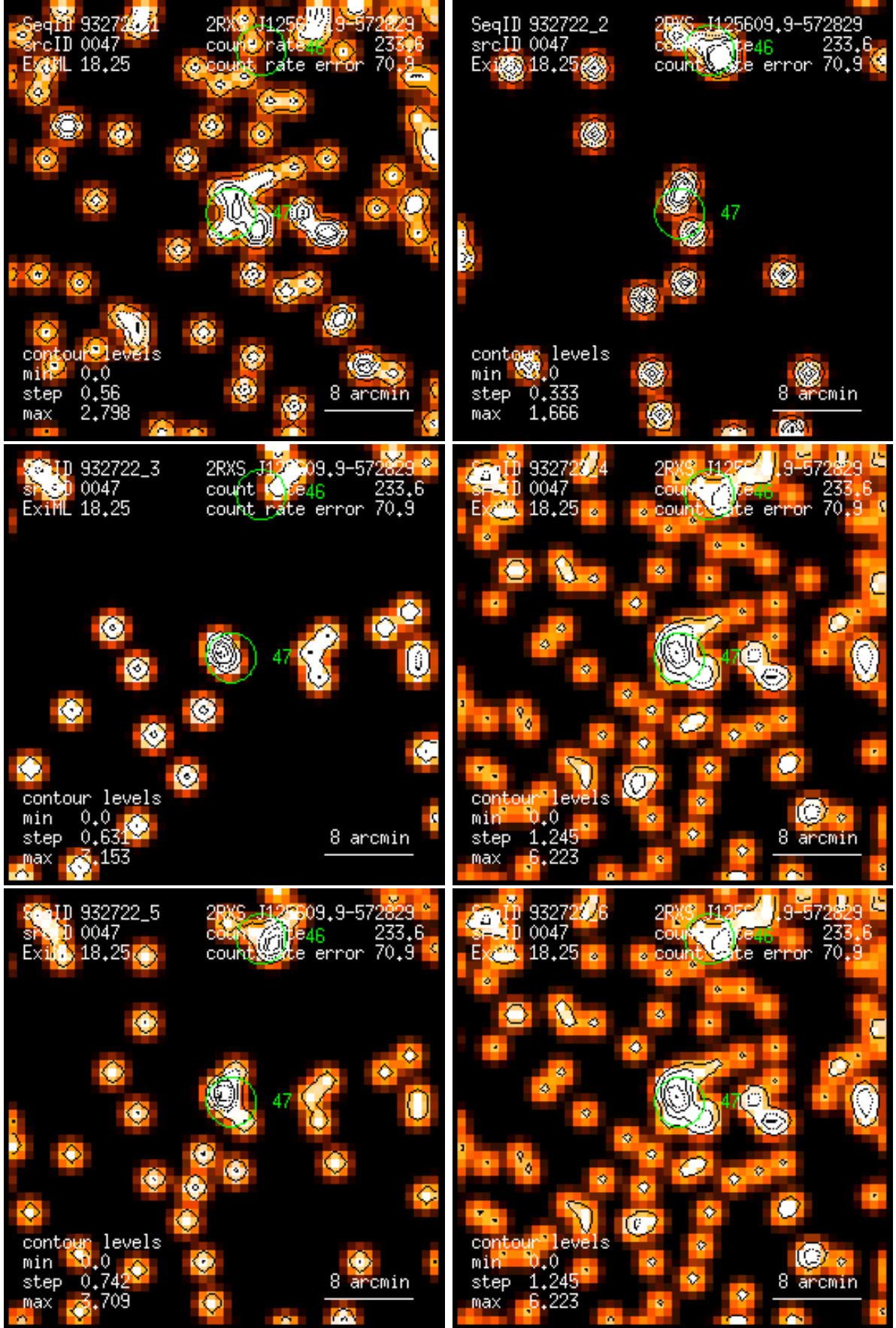
Figure 47: RASS 932722: detection 0047: band rate images, Gaussian filter: (1) PSPC channels 11 – 41, (2) 52 – 90, (3) 91 – 201, (4) 11 – 235, (5) 52 – 201, (6) 11 – 201. Broad band rates in counts/ks. Band rate contour levels in counts/ks/arcmin 2 .
