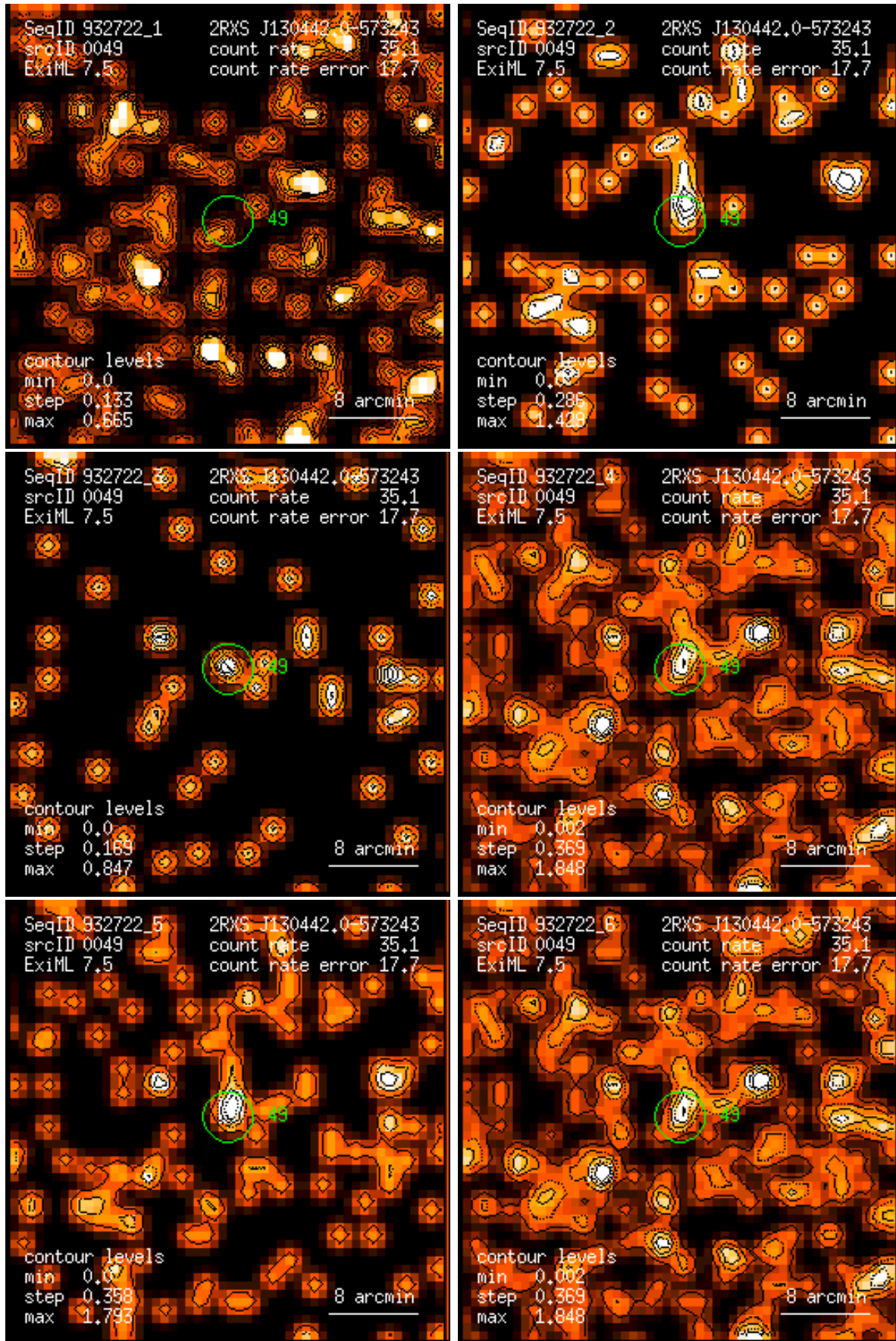
Figure 49: RASS 932722: detection 0049: band rate images, Gaussian filter: (1) PSPC channels 11 – 41, (2) 52 – 90, (3) 91 – 201, (4) 11 – 235, (5) 52 – 201, (6) 11 – 201. Broad band rates in counts/ks. Band rate contour levels in counts/ks/arcmin 2 .
