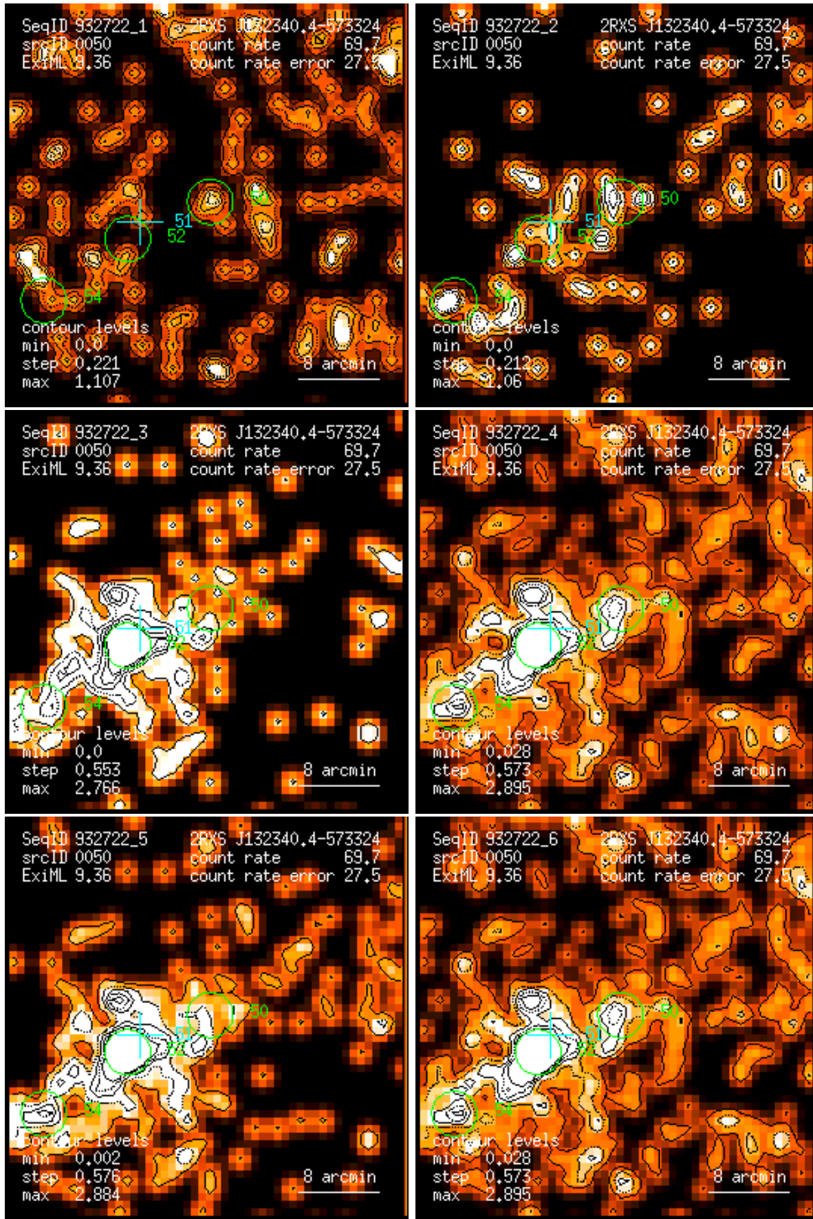
Figure 50: RASS 932722: detection 0050: band rate images, Gaussian filter: (1) PSPC channels 11 – 41, (2) 52 – 90, (3) 91 – 201, (4) 11 – 235, (5) 52 – 201, (6) 11 – 201. Broad band rates in counts/ks. Band rate contour levels in counts/ks/arcmin 2 .
