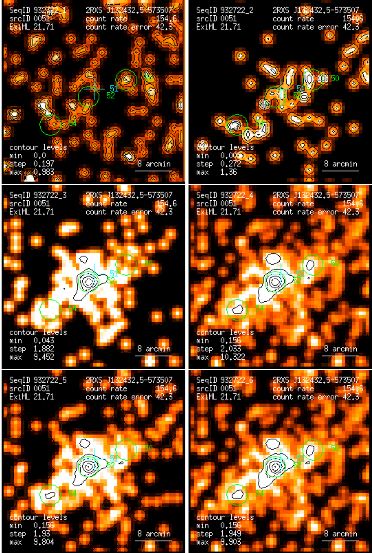
Figure 51: RASS 932722: detection 0051: band rate images, Gaussian filter: (1) PSPC channels 11 – 41, (2) 52 – 90, (3) 91 – 201, (4) 11 – 235, (5) 52 – 201, (6) 11 – 201. Broad band rates in counts/ks. Band rate contour levels in counts/ks/arcmin 2 .
