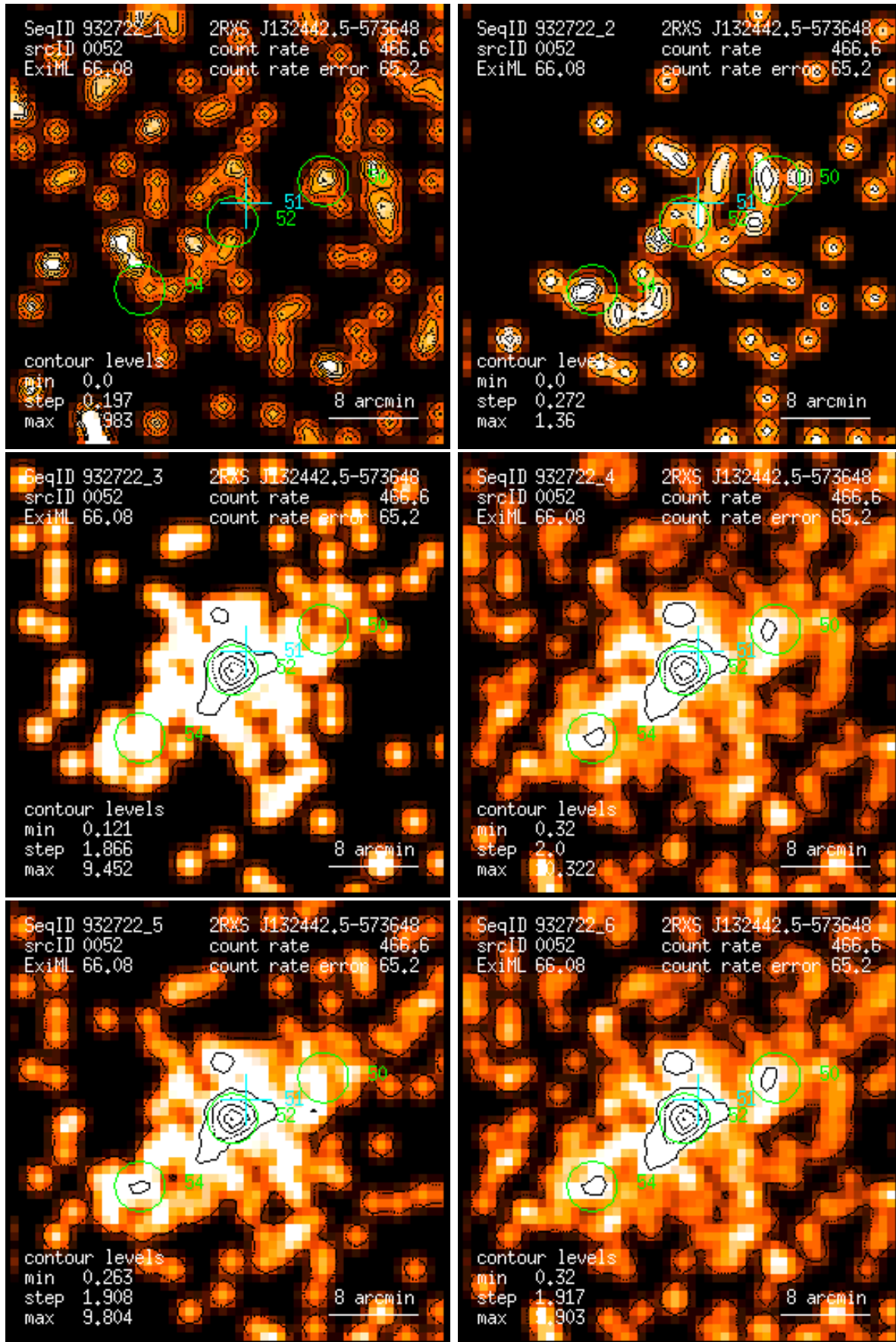
Figure 52: RASS 932722: detection 0052: band rate images, Gaussian filter: (1) PSPC channels 11 – 41, (2) 52 – 90, (3) 91 – 201, (4) 11 – 235, (5) 52 – 201, (6) 11 – 201. Broad band rates in counts/ks. Band rate contour levels in counts/ks/arcmin 2 .
