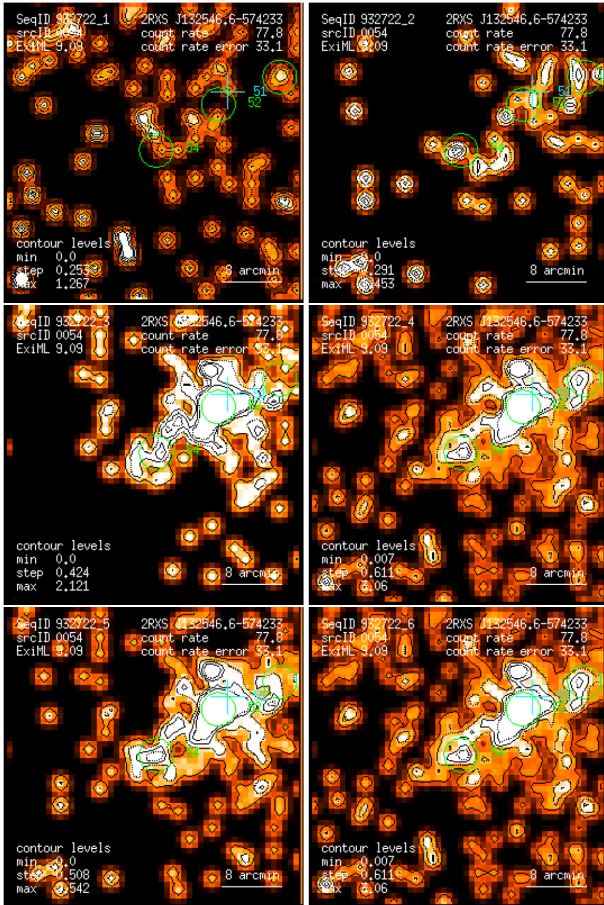
Figure 54: RASS 932722: detection 0054: band rate images, Gaussian filter: (1) PSPC channels 11 – 41, (2) 52 – 90, (3) 91 – 201, (4) 11 – 235, (5) 52 – 201, (6) 11 – 201. Broad band rates in counts/ks. Band rate contour levels in counts/ks/arcmin 2 .
