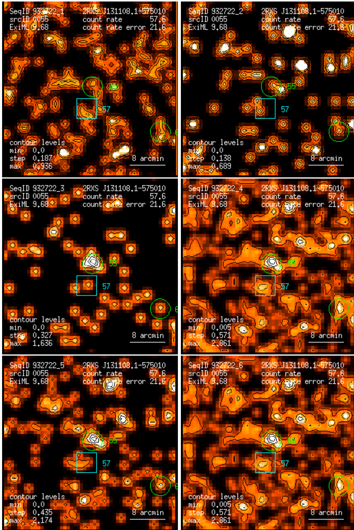
Figure 55: RASS 932722: detection 0055: band rate images, Gaussian filter: (1) PSPC channels 11 – 41, (2) 52 – 90, (3) 91 – 201, (4) 11 – 235, (5) 52 – 201, (6) 11 – 201. Broad band rates in counts/ks. Band rate contour levels in counts/ks/arcmin 2 .
