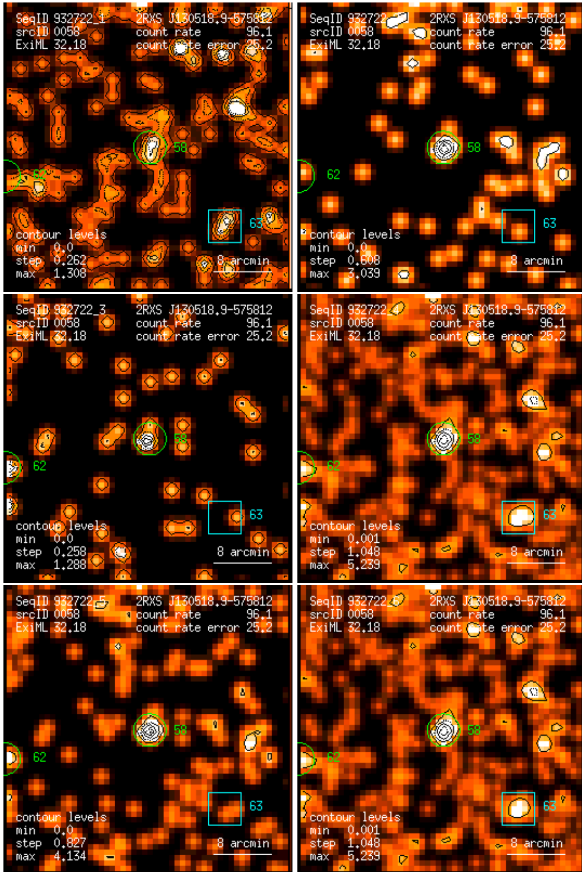
Figure 58: RASS 932722: detection 0058: band rate images, Gaussian filter: (1) PSPC channels 11 – 41, (2) 52 – 90, (3) 91 – 201, (4) 11 – 235, (5) 52 – 201, (6) 11 – 201. Broad band rates in counts/ks. Band rate contour levels in counts/ks/arcmin 2 .
