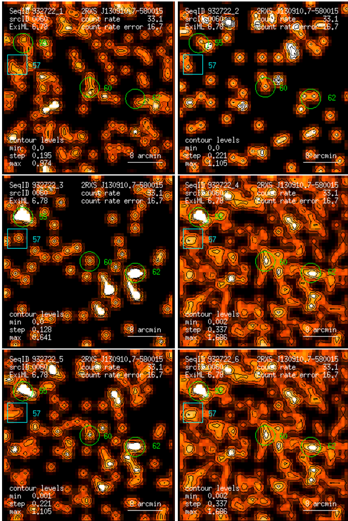
Figure 60: RASS 932722: detection 0060: band rate images, Gaussian filter: (1) PSPC channels 11 – 41, (2) 52 – 90, (3) 91 – 201, (4) 11 – 235, (5) 52 – 201, (6) 11 – 201. Broad band rates in counts/ks. Band rate contour levels in counts/ks/arcmin 2 .
