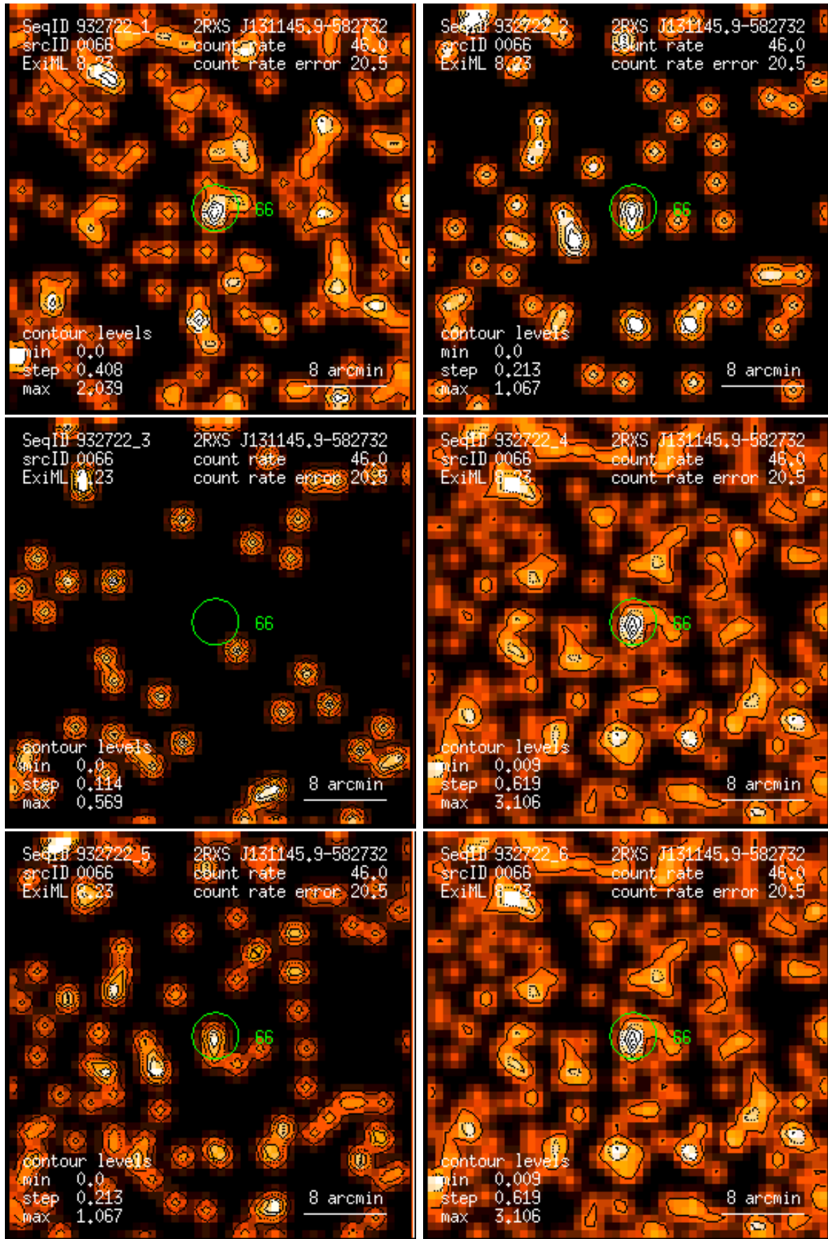
Figure 66: RASS 932722: detection 0066: band rate images, Gaussian filter: (1) PSPC channels 11 – 41, (2) 52 – 90, (3) 91 – 201, (4) 11 – 235, (5) 52 – 201, (6) 11 – 201. Broad band rates in counts/ks. Band rate contour levels in counts/ks/arcmin 2 .
