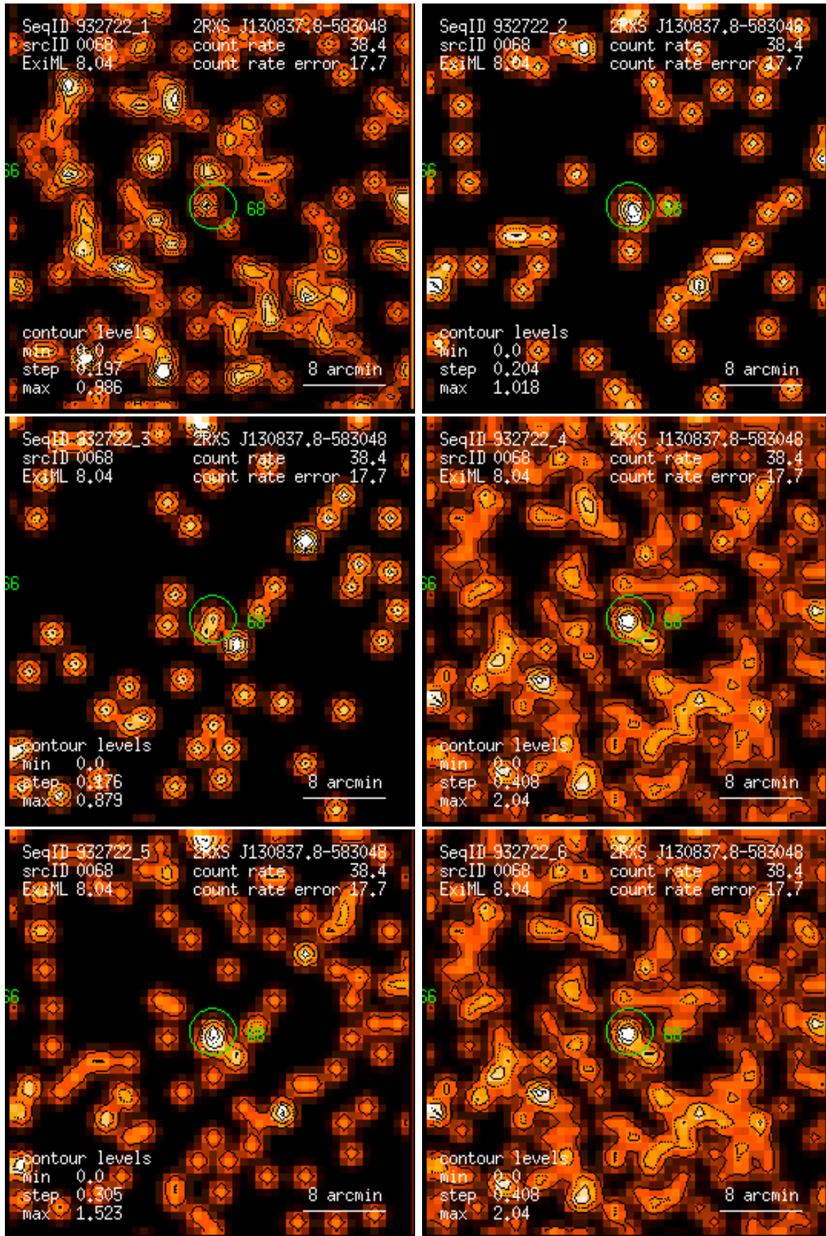
Figure 68: RASS 932722: detection 0068: band rate images, Gaussian filter: (1) PSPC channels 11 – 41, (2) 52 – 90, (3) 91 – 201, (4) 11 – 235, (5) 52 – 201, (6) 11 – 201. Broad band rates in counts/ks. Band rate contour levels in counts/ks/arcmin 2 .
